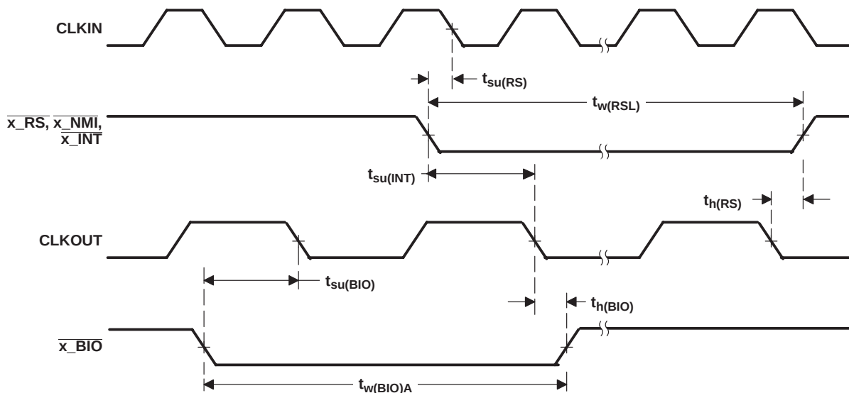
Figure 5–4. Reset and \overline{x\_BIO} Timings
