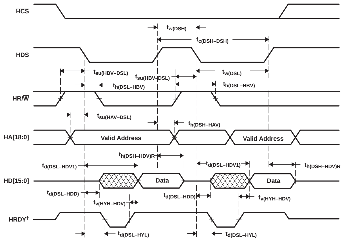
Figure 5–17. Nonmultiplexed Read Timings
