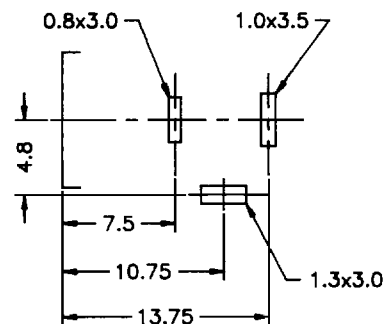
PC BOARD LAYOUT TOP VIEW
