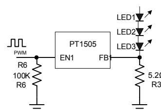
Figure5. Dimming Control Using a PWM Signal
