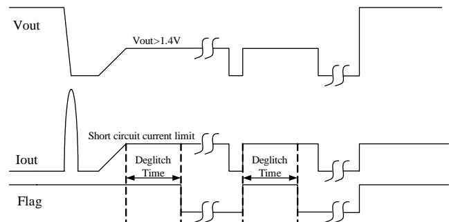
Figure 4—Flag Indication When Short with 1Ω Resistor
