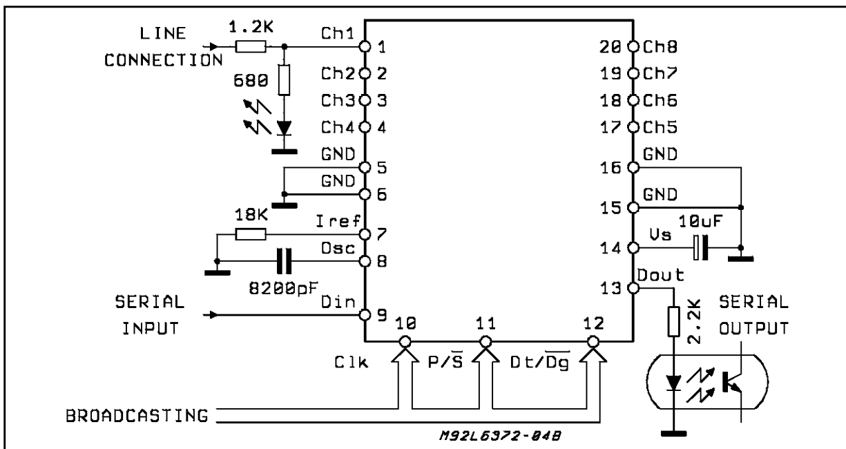
Figure 9: Typical Application
