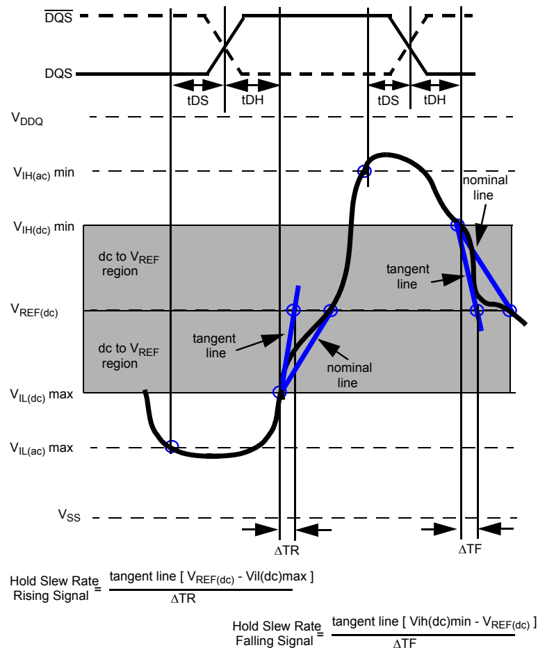
Figure 11 - Illustration of tangent line for t_{\text{DH}} (differential DQS, \overline{\text{DQS}} )
