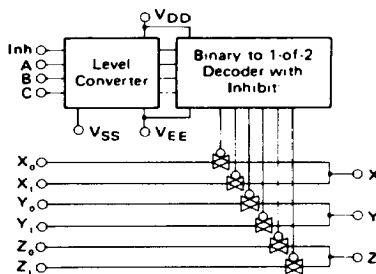
Figure 14 HD14053B Multiplexers/De-Multiplexers
