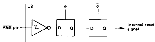
Figure 35 RES circuit
