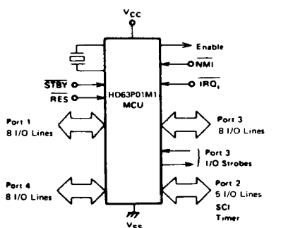
Figure 15 HD63P01M1 MCU Single-Chip Mode
