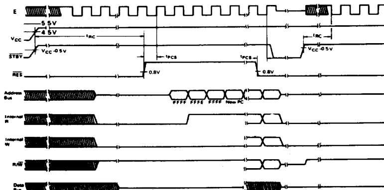
Figure 11 Reset Timing
