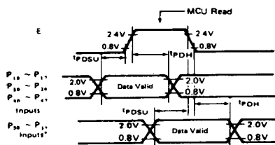
Figure 3 Port Data Set-up and Hold Times (MCU Read)
