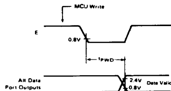
Figure 4 Port Data Delay Times (MCU Write)
