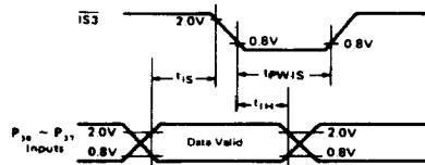
Figure 6 Port 3 Latch Timing (Single Chip Mode)
