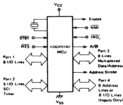
Figure 16 HD63P01M1 MCU Expanded Multiplexed Mode
