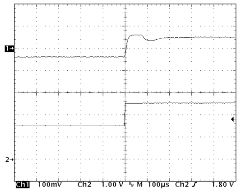
( V_{IN} = 1.5\text{ V to } 2.5\text{ V} ; L = 5.6\text{ }\mu\text{H} , C_{OUT} = 22\text{ }\mu\text{F} , I_{LOAD} = 100\text{ mA} ) Upper Trace: Output Voltage Ripple, 100 mV/Division Lower Trace: Battery Voltage, V_{IN} , 1.0 V/Division
