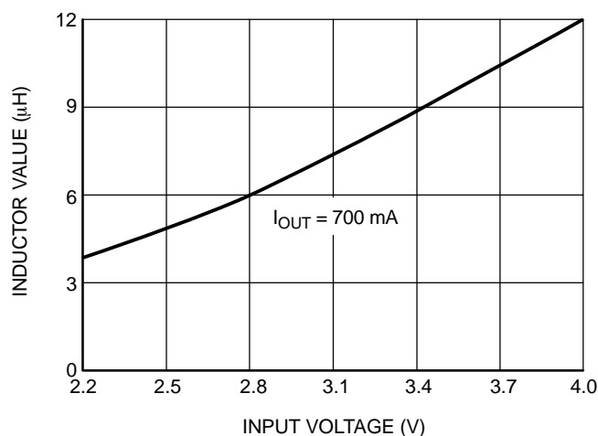
Figure 25. Suggested Inductance of V_{OUT} = 5.0\text{ V}
