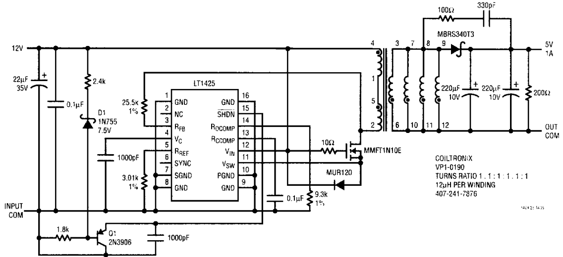
12V to 5V Isolated Converter
