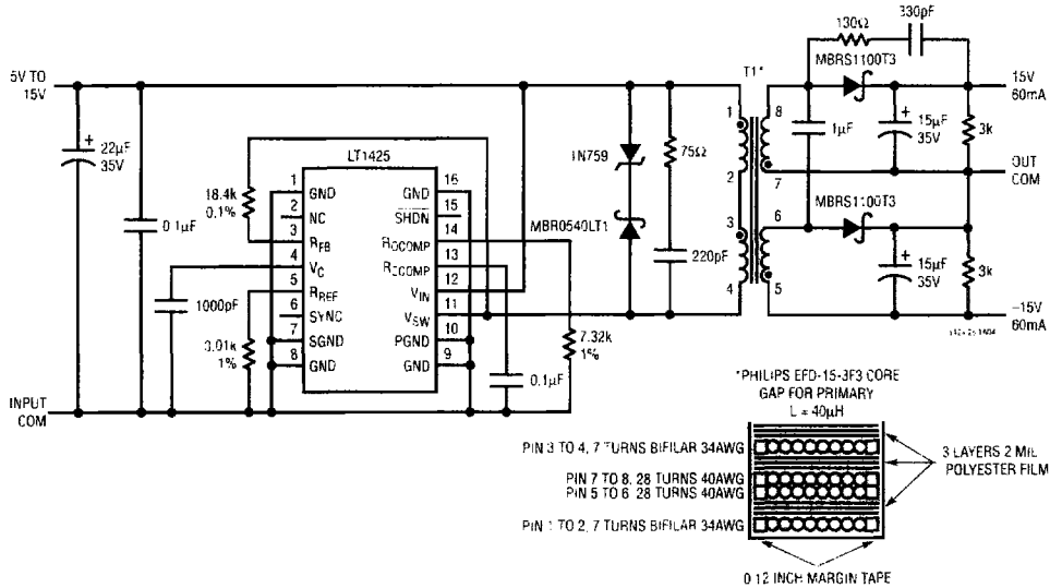
±15V Isolated Power Supply
