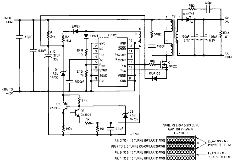
-48V to 5V Isolated Telecom Supply
