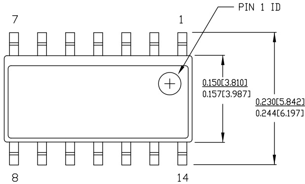
Figure 7. 14-pin (150-Mil) SOIC
