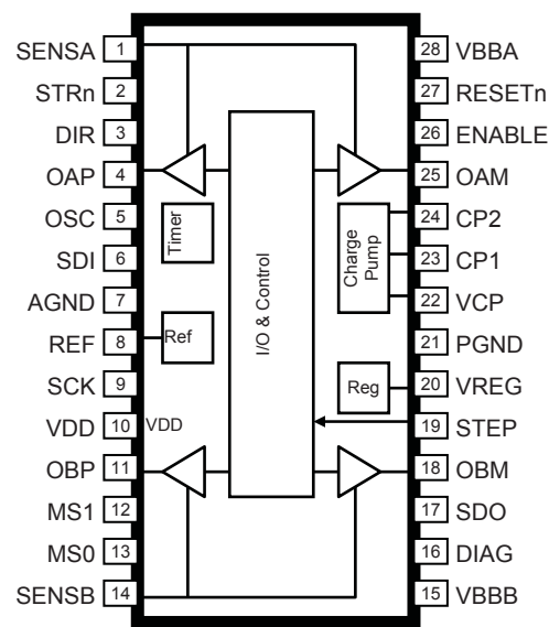
Pin-out Diagram
