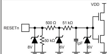
Figure 19g. RESETn Input
