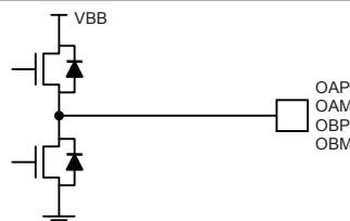
Figure 19i. Phase Outputs
