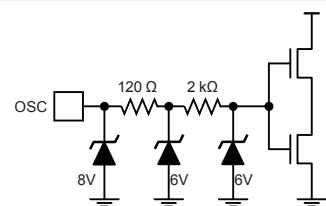
Figure 19f. OSC Input
