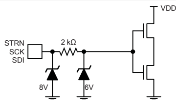
Figure 19e. STRN, SCK, SDI Inputs
