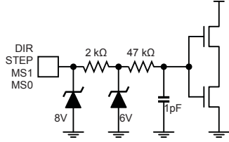
Figure 19c. DIR, STEP, MS1, MS0 Inputs
