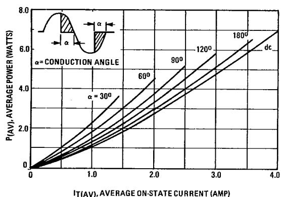
FIGURE 3 - POWER DISSIPATION
