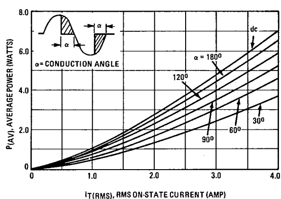
FIGURE 4 - POWER DISSIPATION
