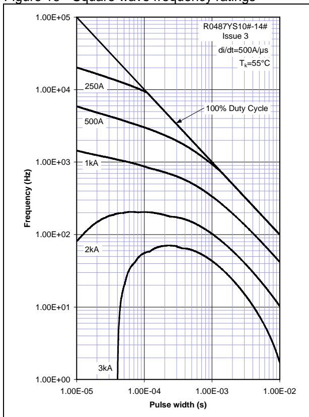
Figure 16 - Square wave frequency ratings
