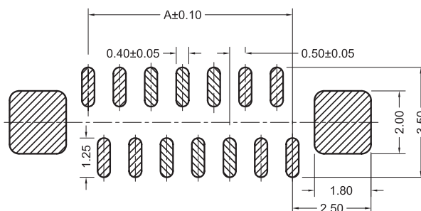
V1 and V2 PCB Layout Reference
