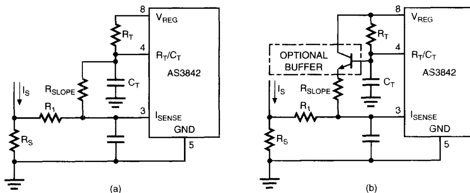
Figure 23. Slope Compensation
