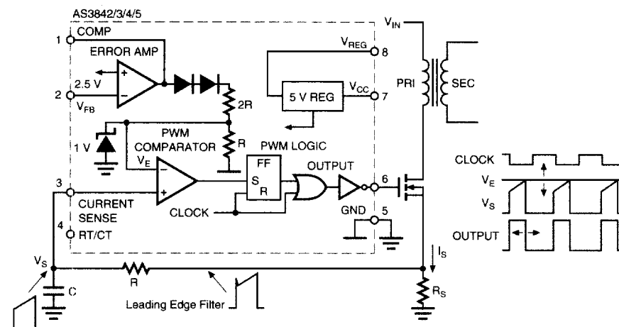
Figure 20. Current Sense/PWM Latch Circuit and Waveforms
