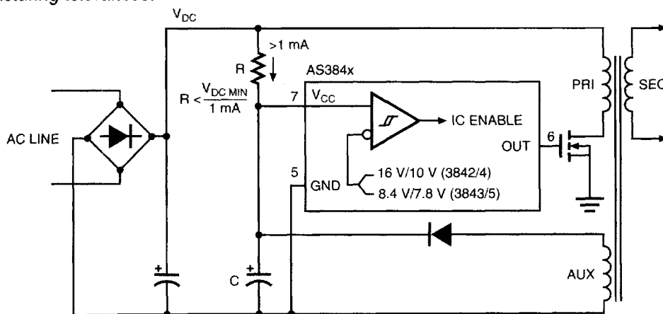
Figure 14. Bootstrap Circuit
