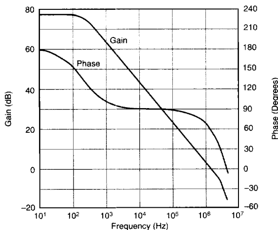
Figure 18. Gain/Phase Response of the AS3842
