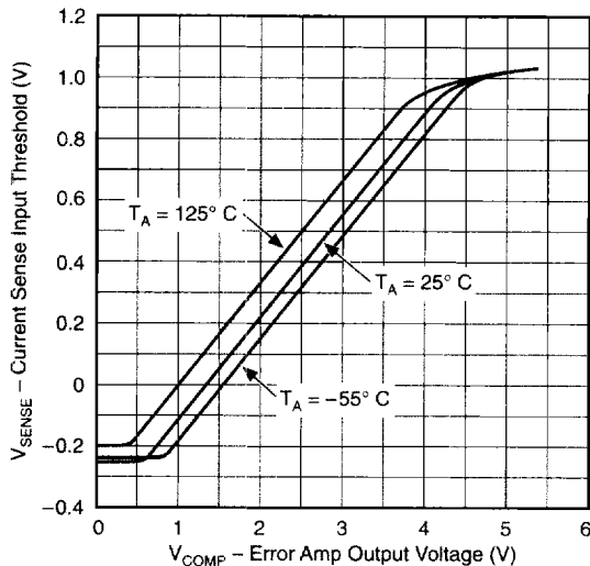
Current Sense Input Threshold vs Error Amp Output Voltage
