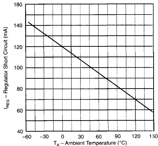
Regulator Short Circuit Current vs Ambient Temperature
