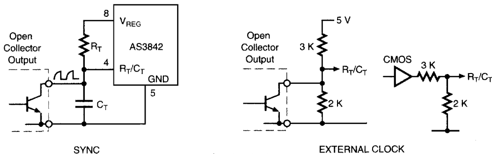
Figure 16. Synchronization
