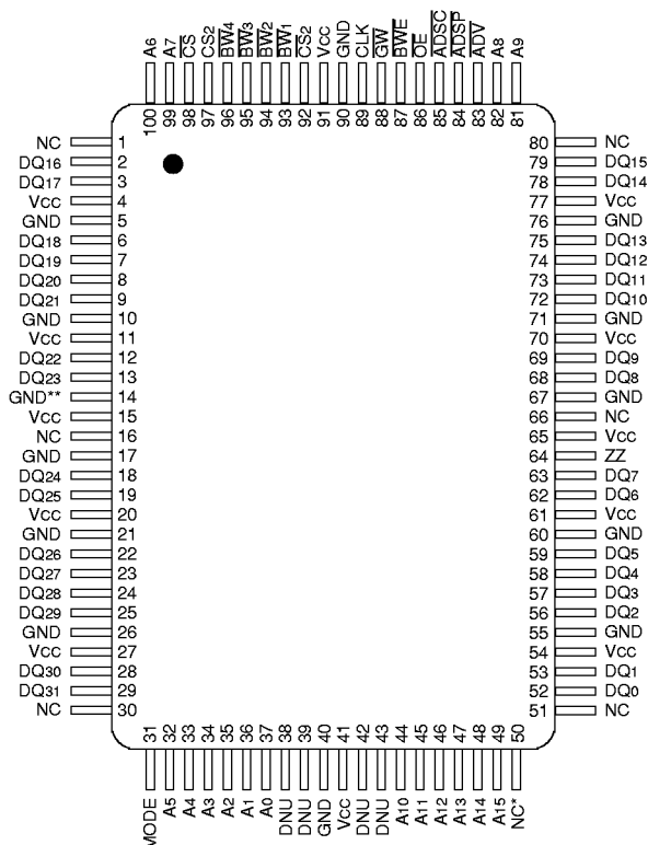
FIG. 1 PIN CONFIGURATION FOR WMY64K32V-XTQX
