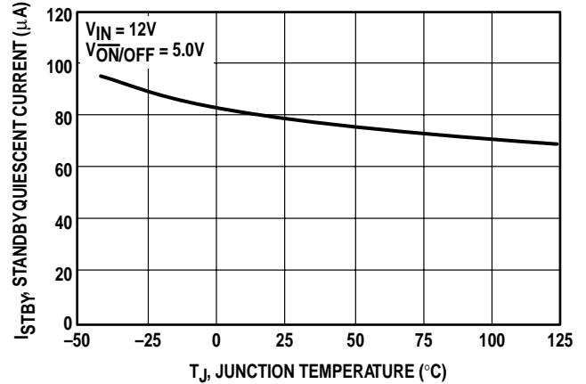
Figure 27. Standby Quiescent Current
