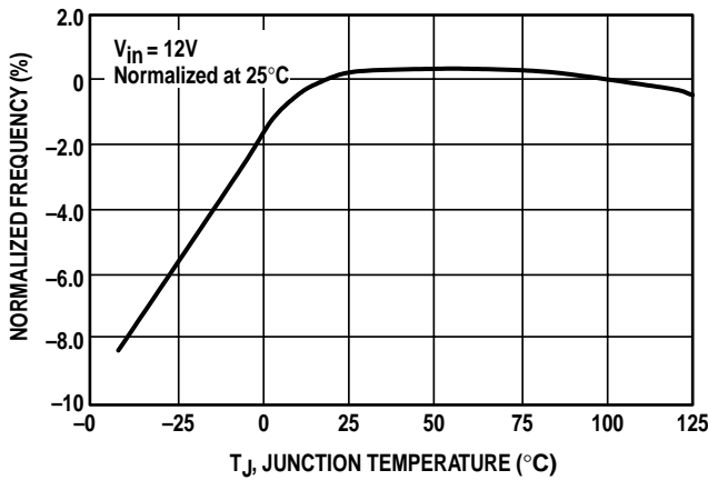
Figure 28. Oscillator Frequency
