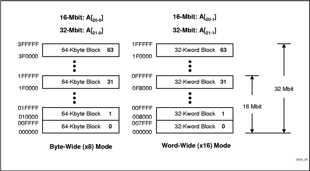
Figure 4. Memory Map
