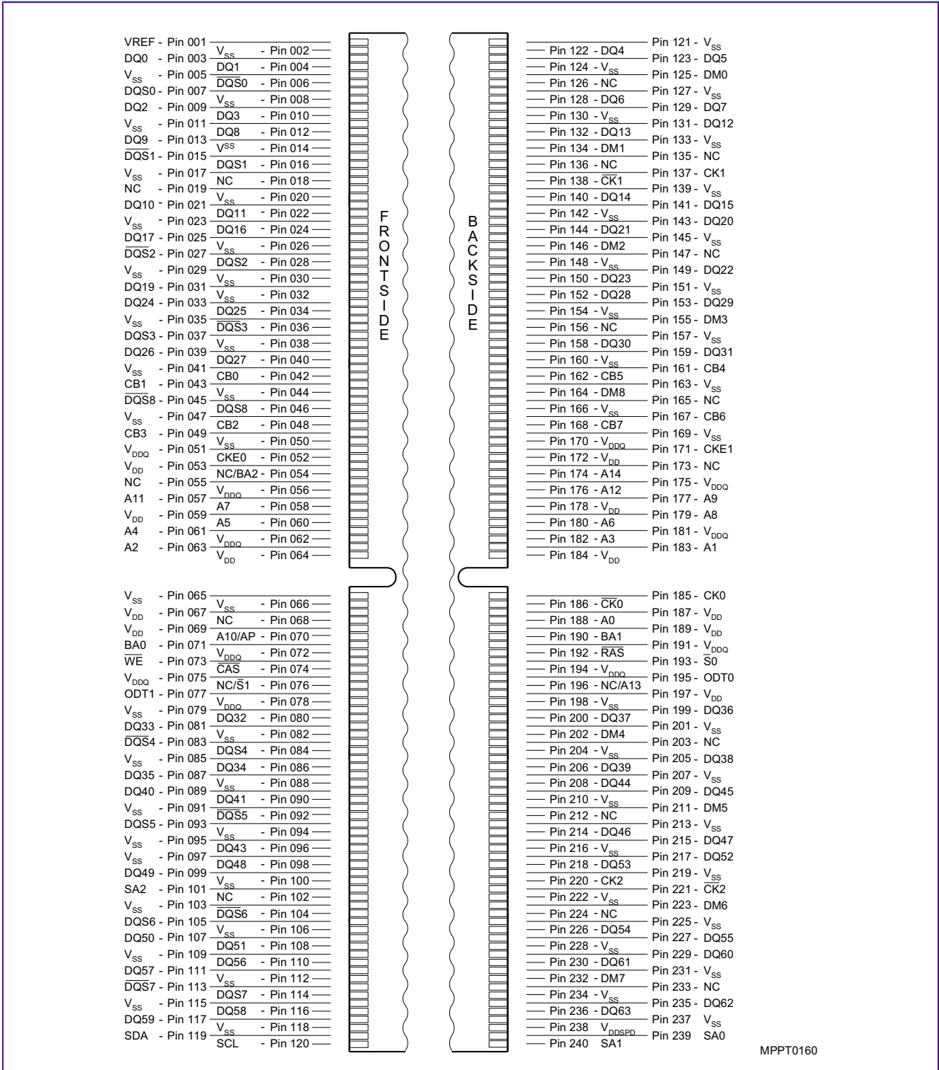
FIGURE 1 Pin Configuration UDIMM ×72 (240 Pin)
