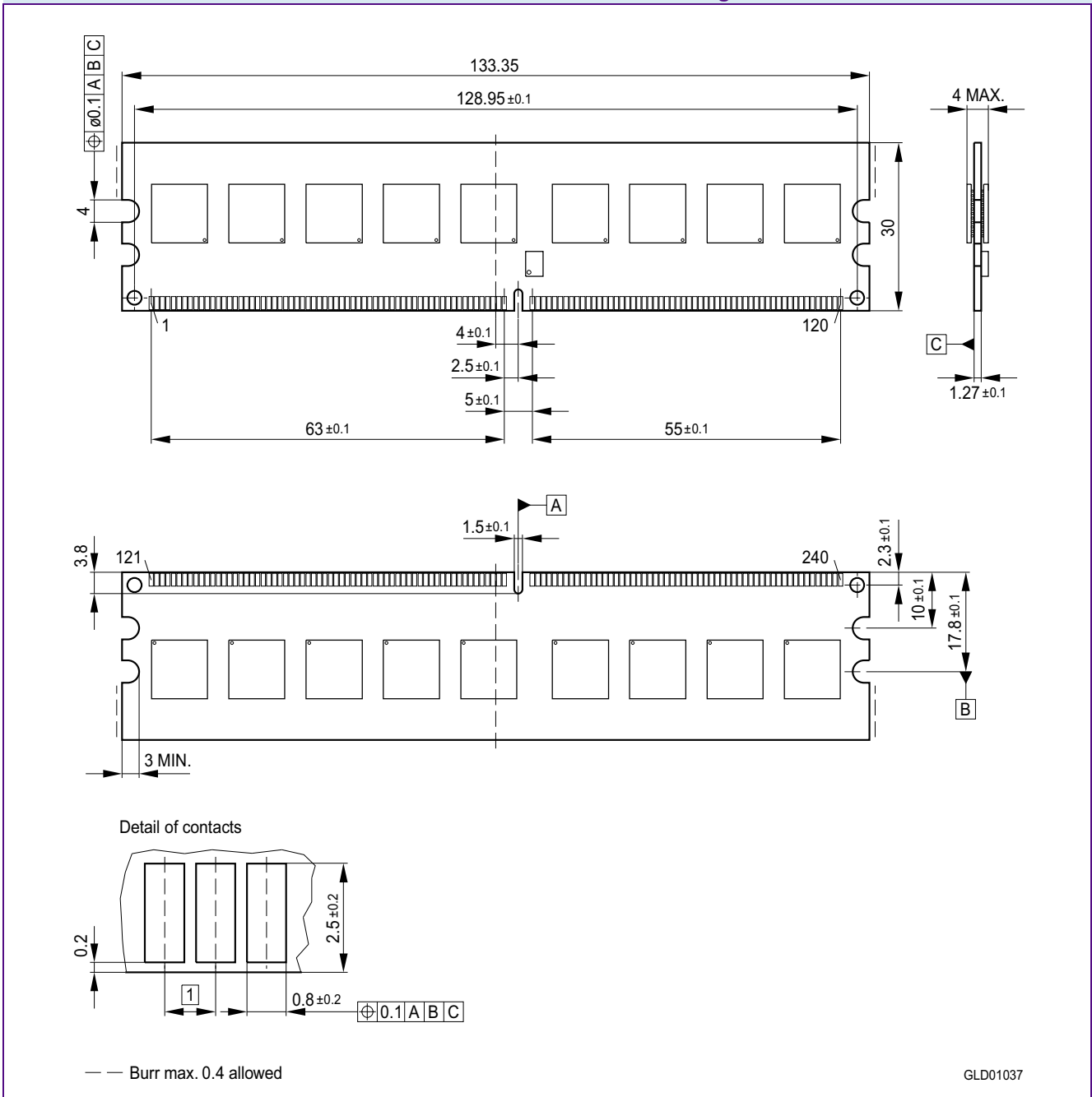
FIGURE 8 Package Outline L-DIM-240-7 Raw Card G
