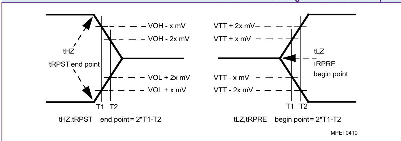
FIGURE 3 Method for Calculating Transitions and Endpoint
