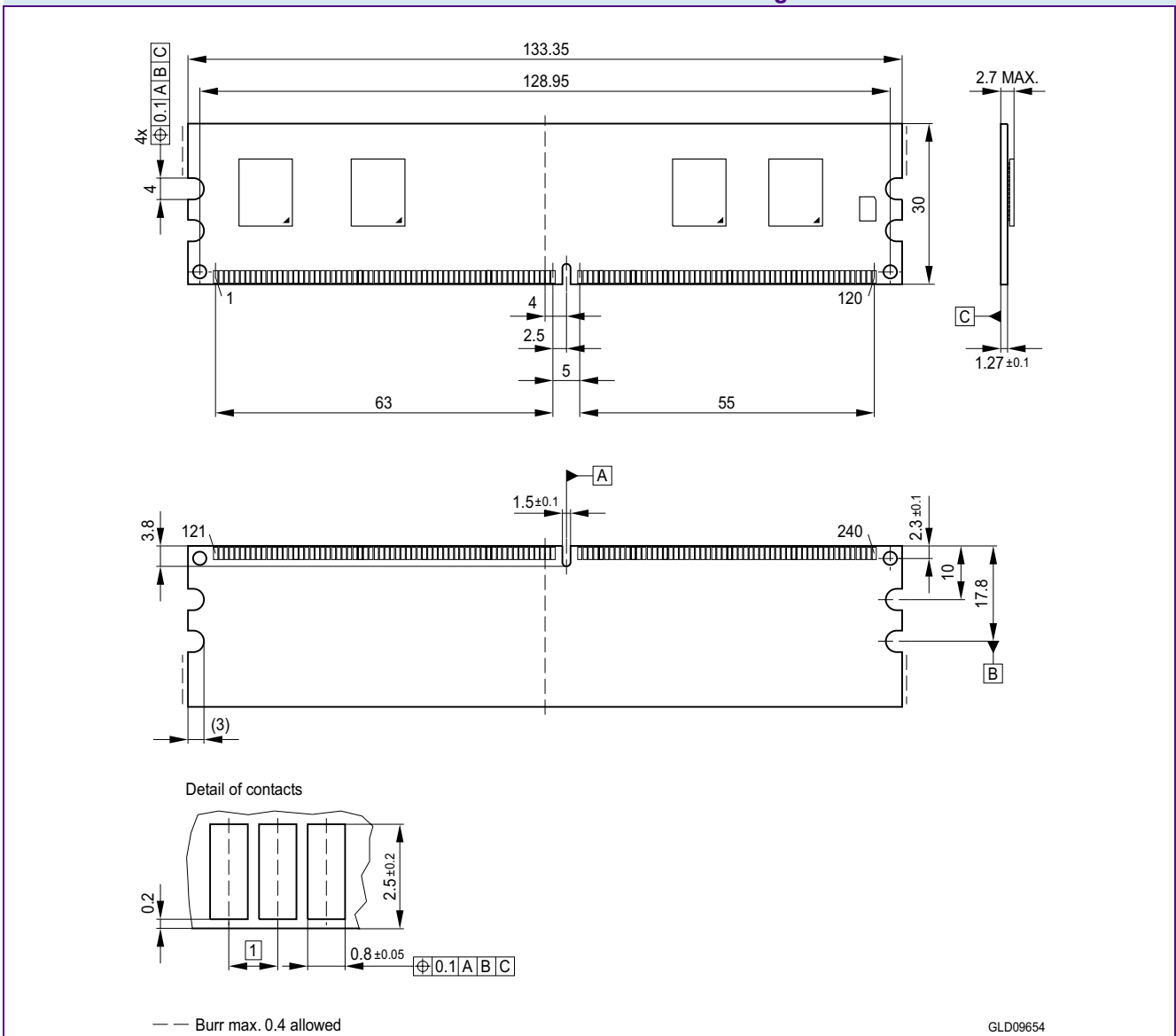
FIGURE 6 Package Outline L-DIM-240-3 Raw Card C
