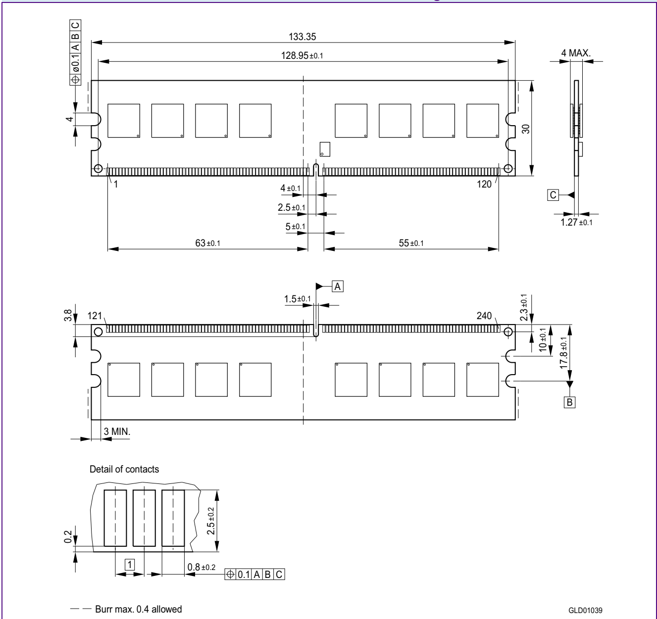
FIGURE 10 Package Outline L-DIM-240-9 Raw Card E
