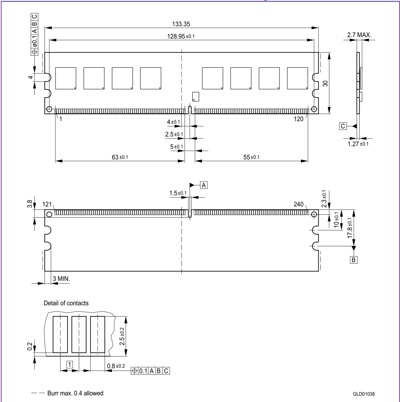
FIGURE 9 Package Outline L-DIM-240-8 Raw Card D
