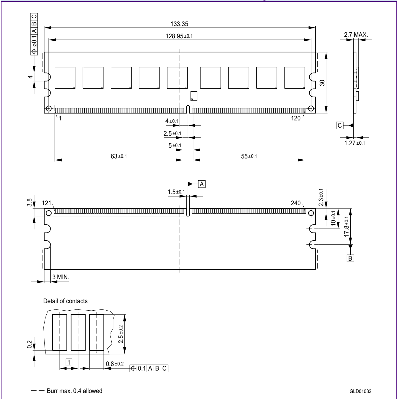
FIGURE 7 Package Outline L-DIM-240-6 Raw Card F
