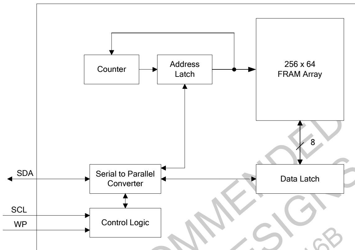
Figure 1. Block Diagram
