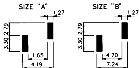
Typical Pad Layout
