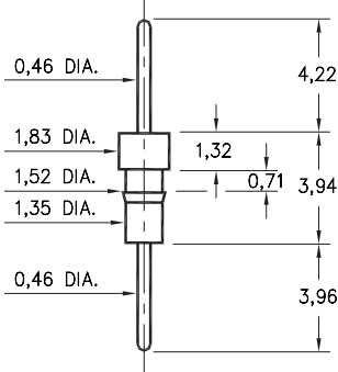
050X-0-00-XX-00-00-03-0 Press-fit in 1,45 mounting hole
