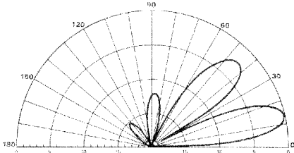
Frequency 10 MHz
