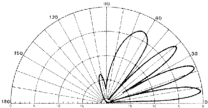
Frequency 18 MHz
