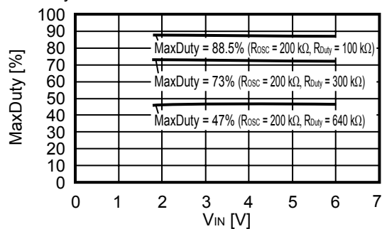
MaxDuty vs. V_{IN}
