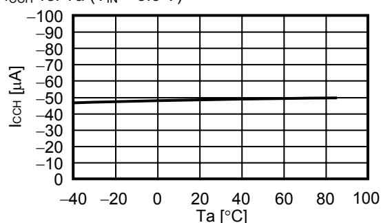
I_{CCH} vs. T_a ( V_{IN} = 3.3 V)
