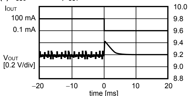
(6) f_{OSC} = 286\text{ kHz} , I_{OUT} = 100\text{ mA} \rightarrow 0.1\text{ mA}
