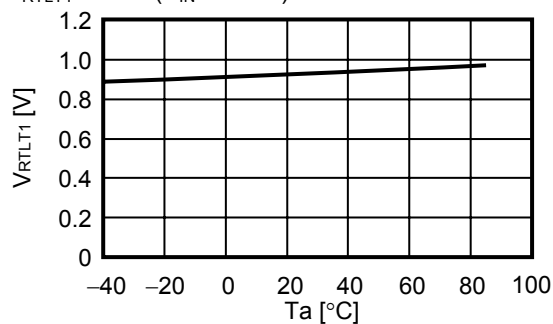
V_{RTL1} vs. T_a ( V_{IN} = 3.3 V)
