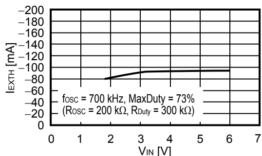
I_{EXTH} vs. V_{IN}
