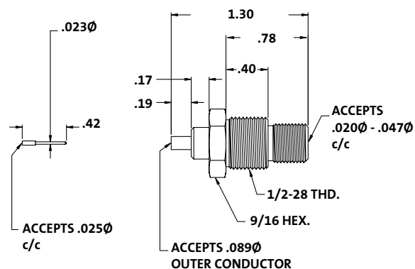
Female Conformable Coax Solder Connector
