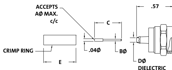
RG-179B/U Coax Connector & RG-179B/U Double Braided Coax Connector
