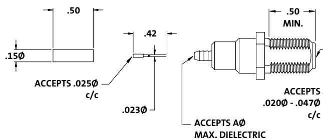
RG-179B/U Female Coax Connector
