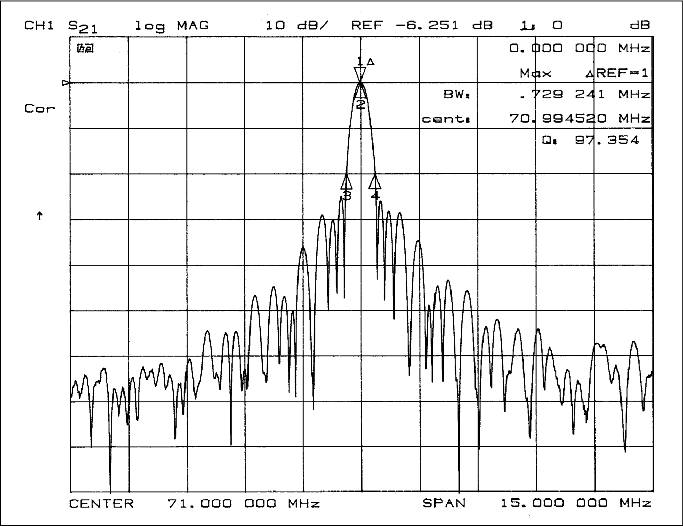
Figure 1: Amplitude Characteristics
