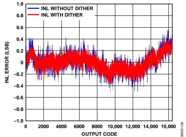
Figure 28. AD9255-105 INL with f_{IN} = 12.5 MHz
