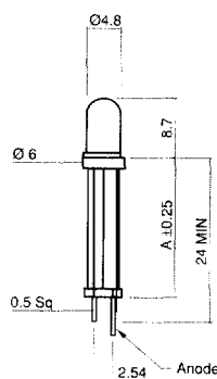
Scale 1 : 1 Dimensions in mm (Typical)
