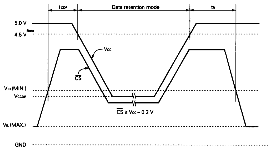
Data Retention Timing Chart
