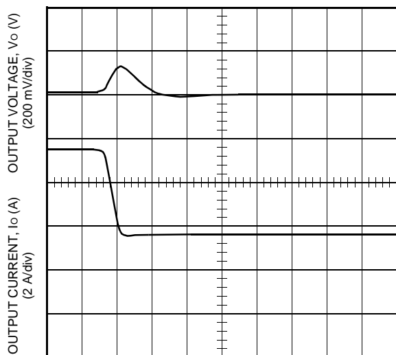
Figure 13. Typical QHW050F1-Q Transient Response to Step Decrease in Load from 50% to 25% of Full Load at Room Temperature and 48 Vdc Input. (Waveform Averaged to Eliminate Ripple Component.)
