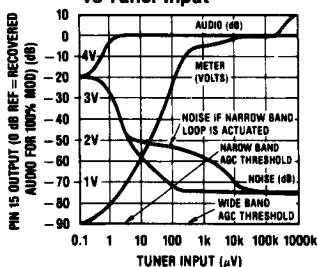
Meter Output and Signal-to-Noise vs Tuner Input
