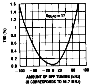
% THD vs OFF Tuning (Single Tuned Quadrature Coil)
