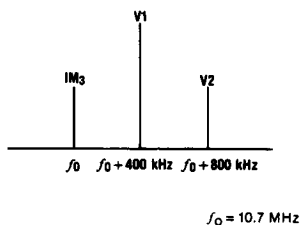
FIGURE 13. Spectrum Analyzer Display of Tuner Output
