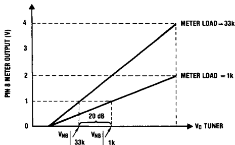
FIGURE 11. Effect of Meter Load on Narrow Band Threshold
