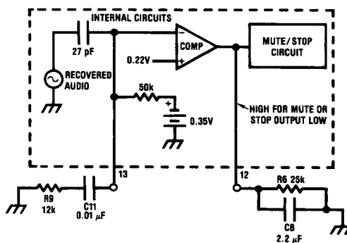
FIGURE 4. Simplified Level Mute/Stop Circuit
