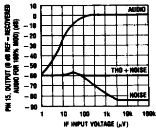
FM Limiting Characteristics + THD
