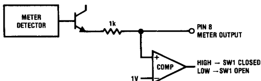
FIGURE 10. Narrow Band Threshold Circuit
