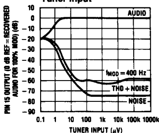
Total Harmonic Distortion vs Tuner Input
