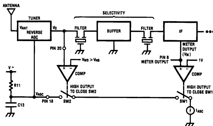
FIGURE 5. Dual Threshold AGC
