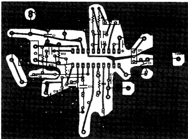
PC Layout (Component Side)
