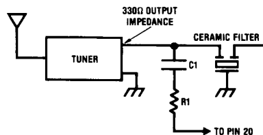
FIGURE 14. Wide Band Threshold Adjustment
