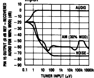
AM Rejection vs Tuner Input
