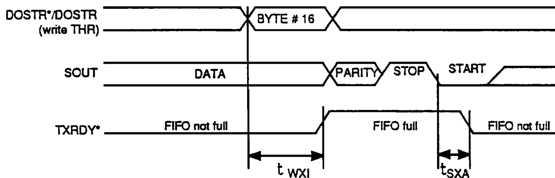
Figure 18 - Transmitter Ready Timing in DMA (FCR0 = 0 or FCR0 = 1 and FCR3 = 0) Mode 1
