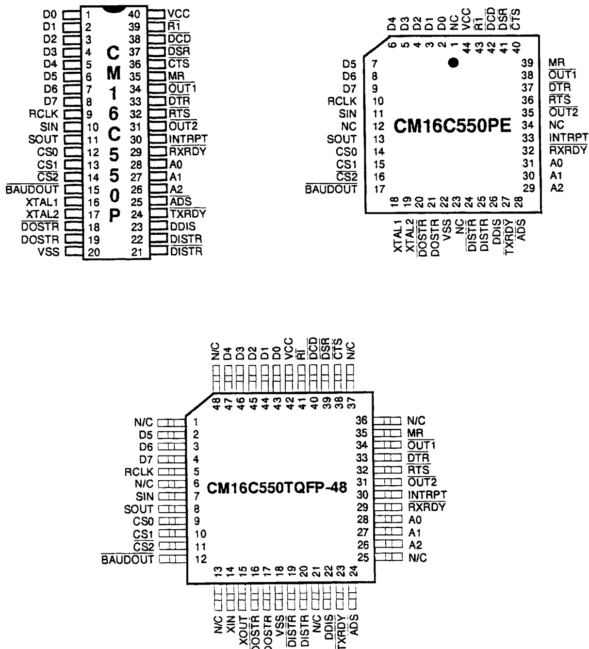
Figure 2 - Pin Configurations
