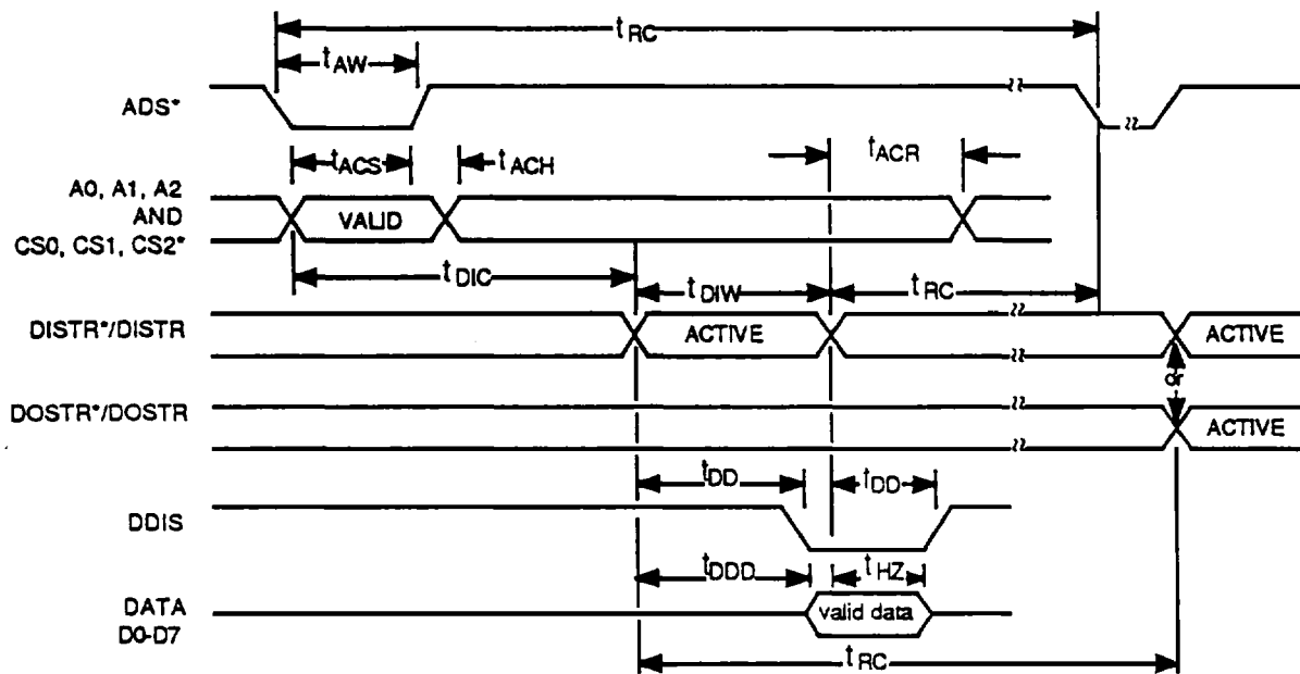
Figure 8 - Read Cycle Timing
