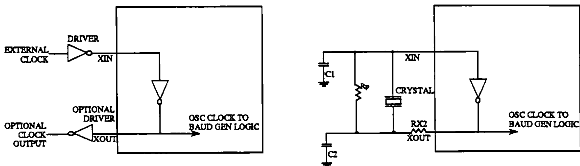
Figure 5 - Typical Crystal Oscillator Network
