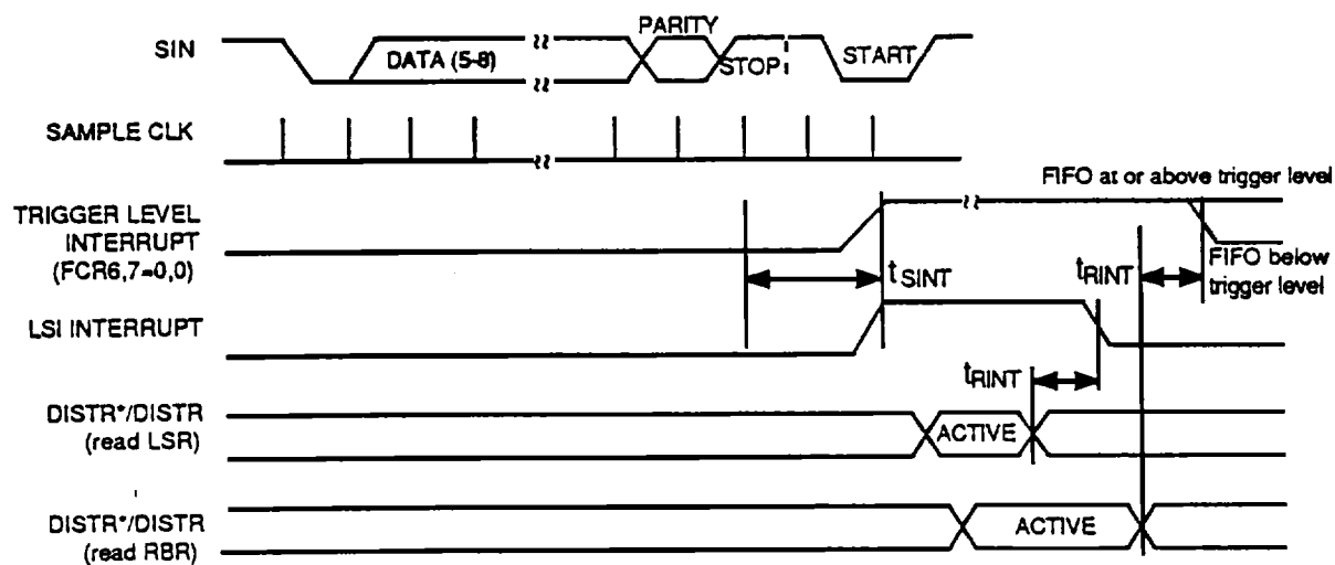
Figure 12 - RCVR FIFO Timing for First Byte
