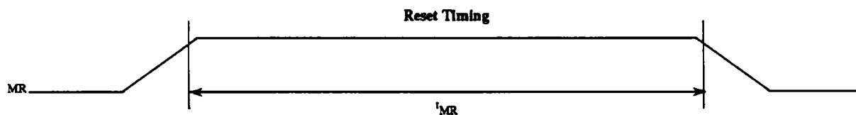
Figure 6 - Clock and Reset Timing
