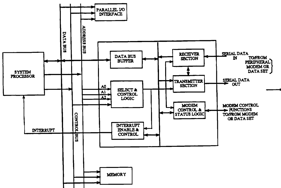
Figure 1 - CM16C550 General System Configuration
