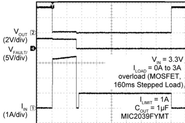
Time (20ms/div)
