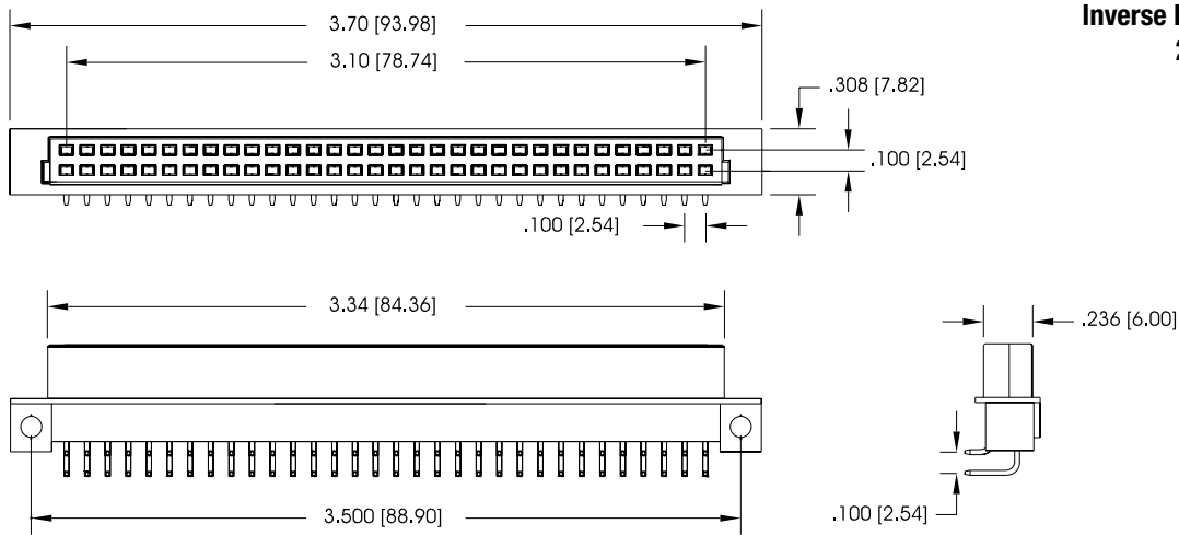
PC Board Layout - Male
