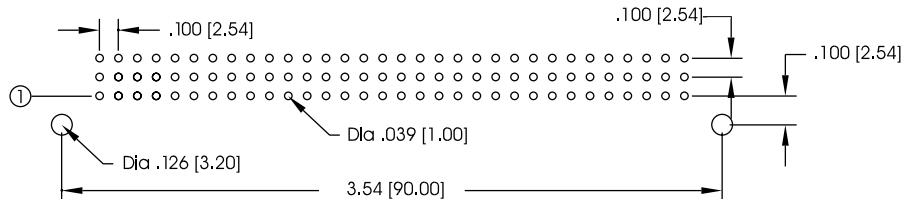
PC Board Layout - Female
