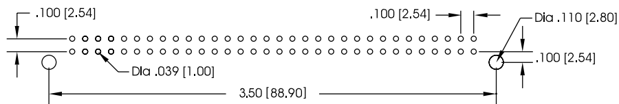
PC Board Layout - Male
