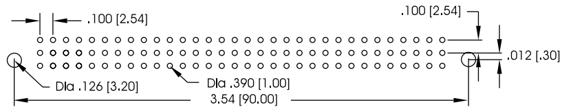
PC Board Layout - Male
