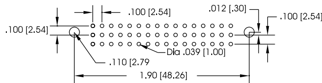
PC Board Layout - Male
