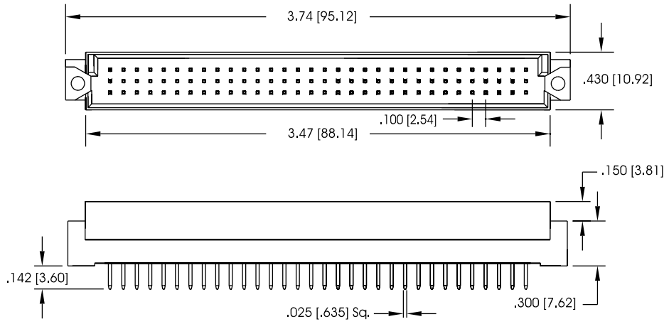
Inverse DIN Type R Male 3 Row Straight M41X-MSXX-051
