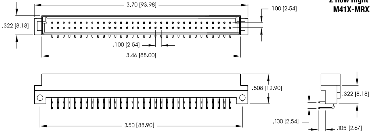
Standard DIN Type B Female 2 Row Straight M41X-FSXX-031
