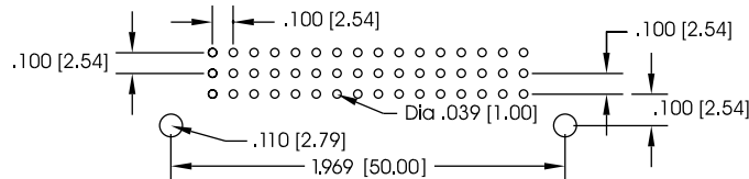
PC Board Layout - Female
