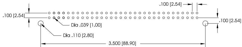
PC Board Layout - Female
