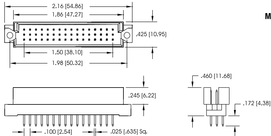
Inverse DIN Type 1/2 R Female 3 Row Right Angle M41X-FRXX-021
