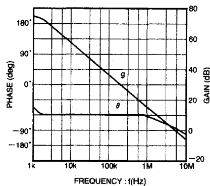
Fig. 8 Operational amplifier vs. open loop characteristics
