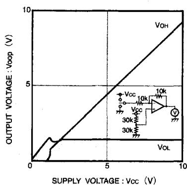
Fig. 7 Supply voltage vs. operational amplifier high/low level output voltage
