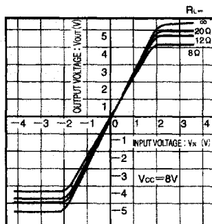
Fig. 4 Drive I/O characteristics (variable load)
