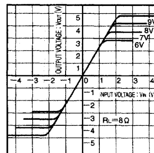
Fig. 5 Drive I/O characteristics (variable supply voltage)
