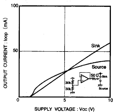
Fig. 6 Supply voltage vs. operational amplifier output current
