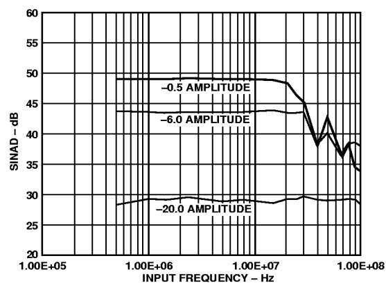
Figure 6. SINAD vs. Input Frequency
