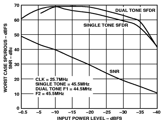
Figure 35. SNR/SFDR for IF @ 45 MHz
