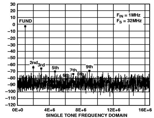
Figure 12. Single-Tone Frequency Domain
