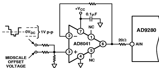
Figure 28. Bipolar Level Shift
