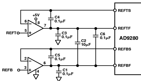
Figure 23b. Kelvin Connected Reference Using the AD9280
