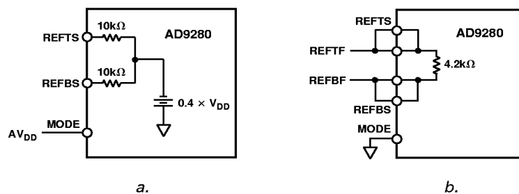
Figure 1. Equivalent Input Load
