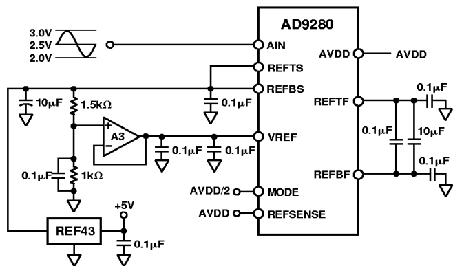
Figure 22. External Reference Mode—1 V p-p Input Span 2.5 V V_{CM}
