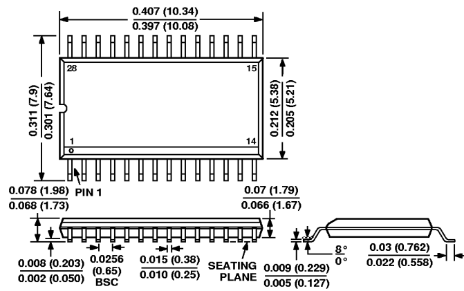
RS-28 28-Lead Shrink Small Outline Package (SSOP)
