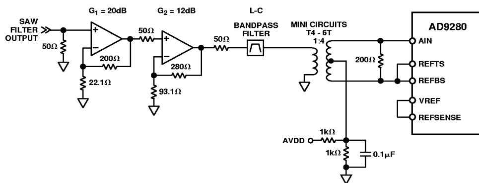
Figure 34. Simplified AD9280 IF Sampling Circuit
