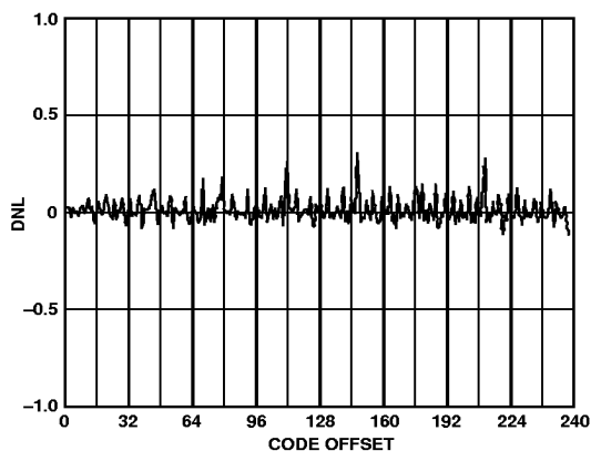
Figure 3. Typical DNL
