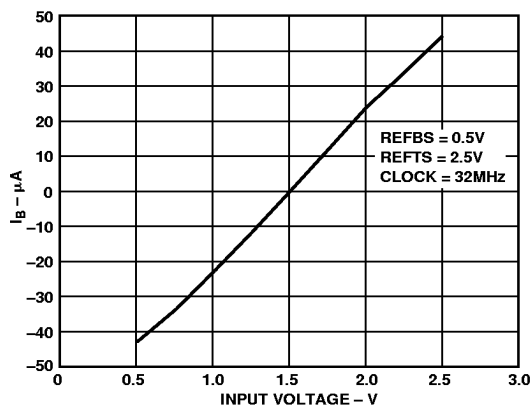
Figure 14. Input Bias Current vs. Input Voltage
