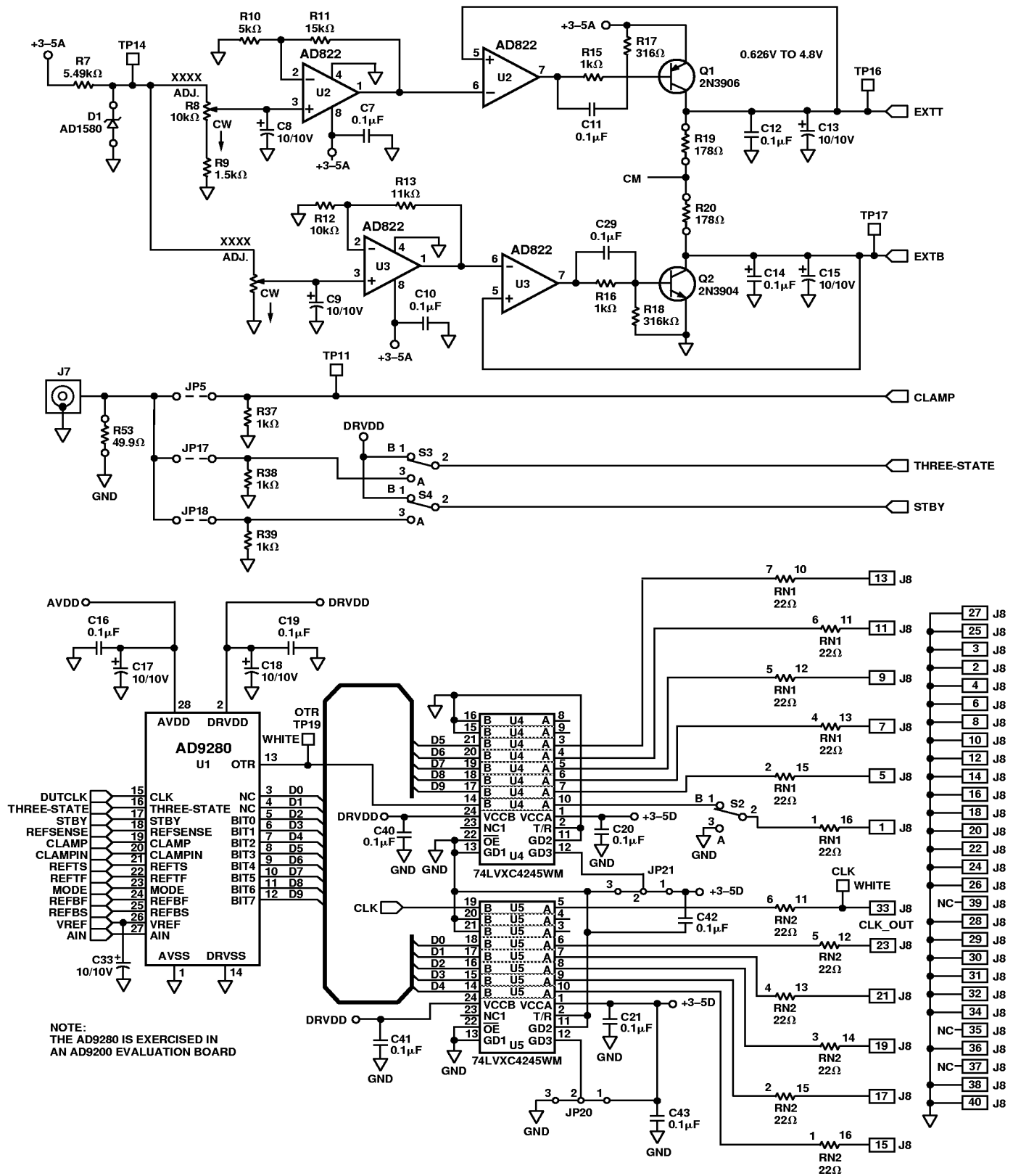
Figure 39a. Evaluation Board Schematic
