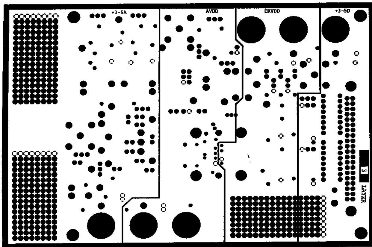
Figure 40c. Evaluation Board Power Plane (Not to Scale)
