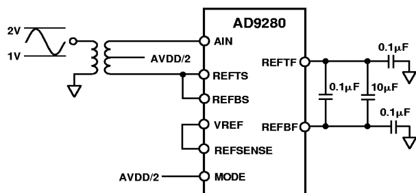
Figure 29. Differential Input
