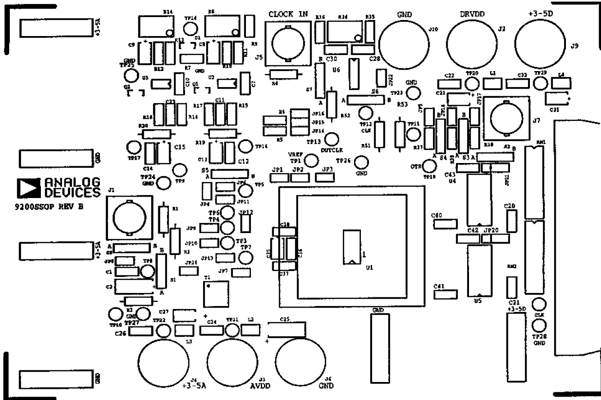
Figure 40e. Evaluation Board Component Silk (Not to Scale)
