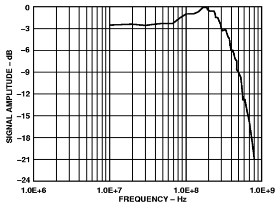
Figure 13. Full Power Bandwidth
