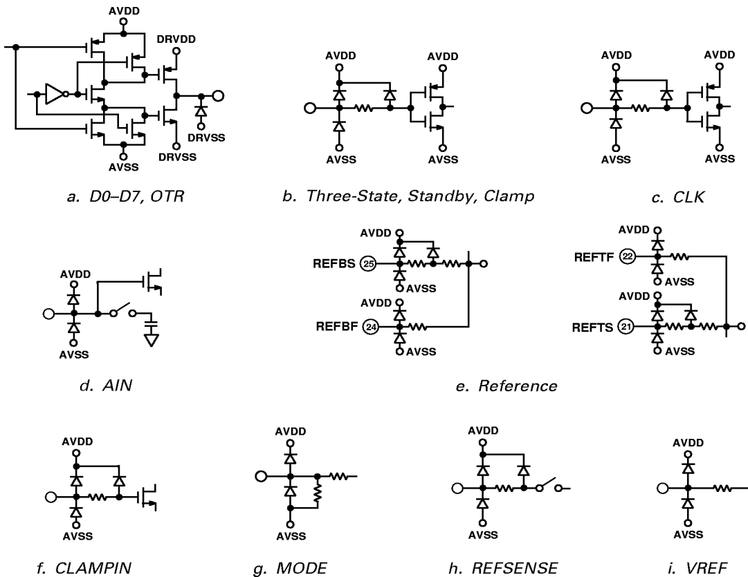
Figure 2. Equivalent Circuits
