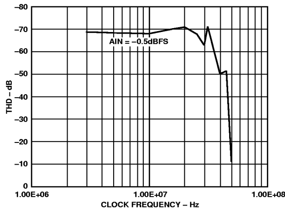
Figure 8. THD vs. Clock Frequency
