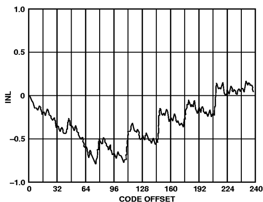
Figure 4. Typical INL
