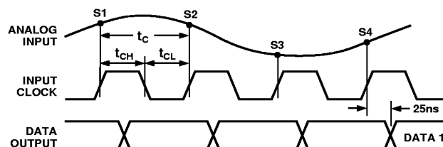
Figure 31. Timing Diagram
