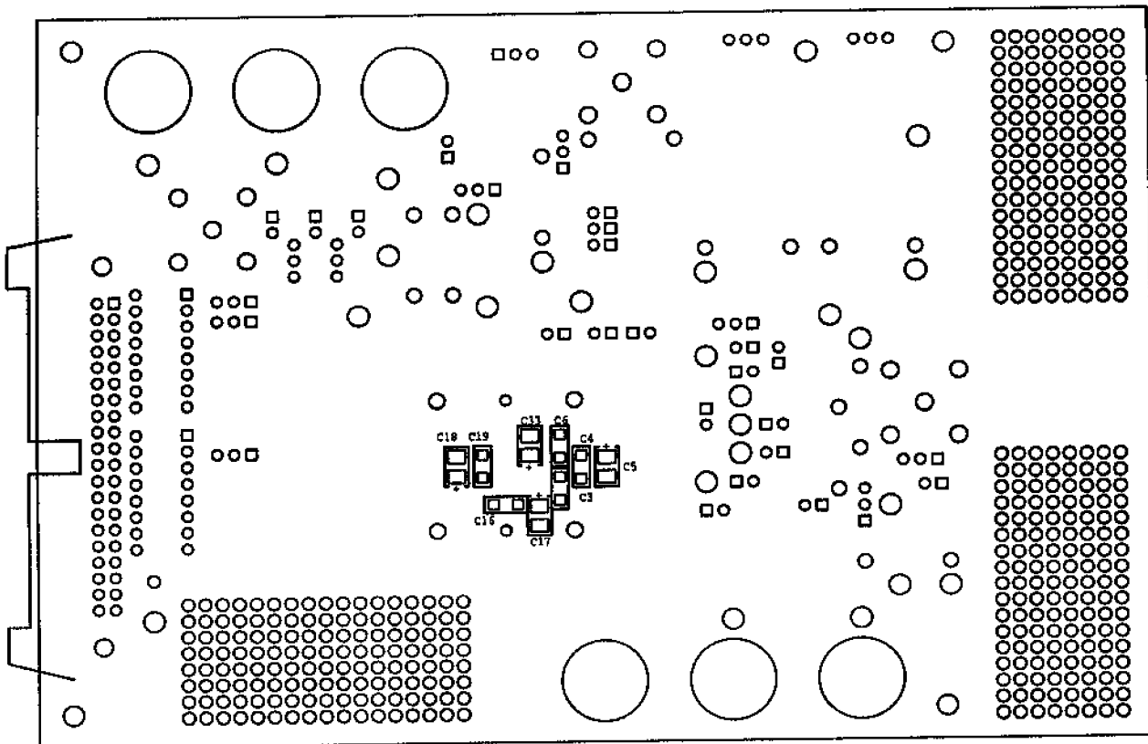
Figure 40f. Evaluation Board Solder Silk (Not to Scale)
