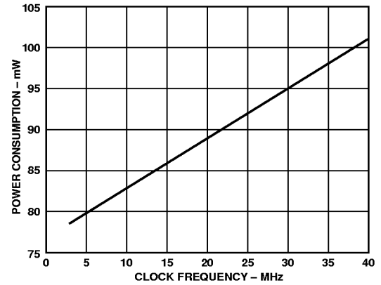
Figure 10. Power Consumption vs. Clock Frequency (MODE = AVSS)
