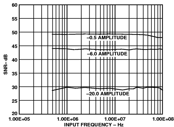
Figure 5. SNR vs. Input Frequency
