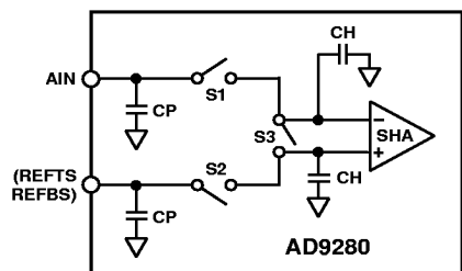
Figure 25. AD9280 Equivalent Input Structure
