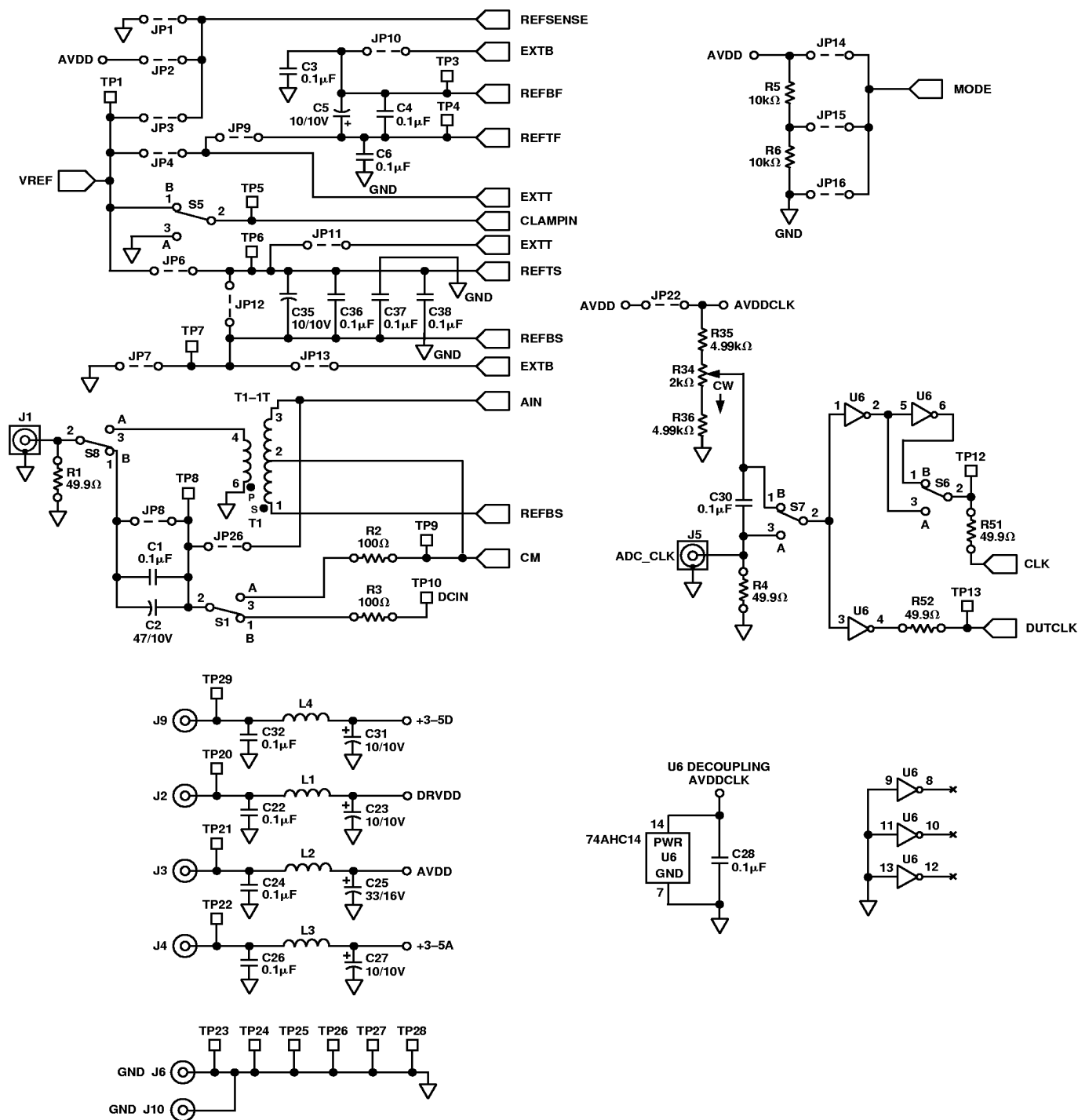
Figure 39b. Evaluation Board Schematic
