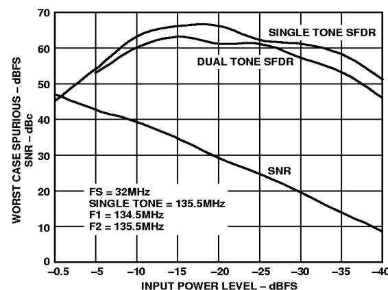
Figure 38. SNR/SFDR for IF @ 135 MHz
