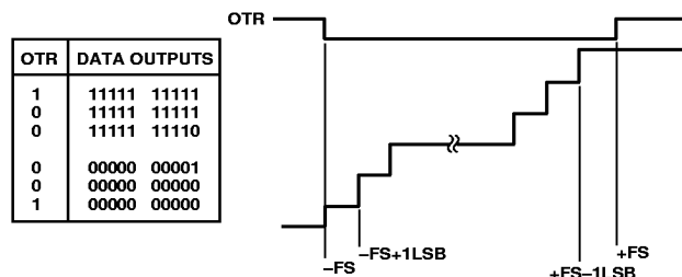
Figure 32. Output Data Format
