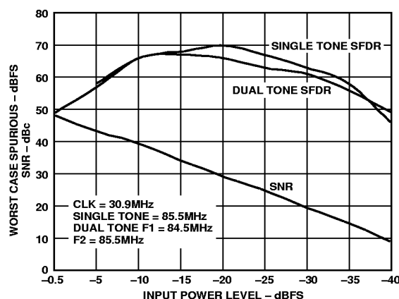
Figure 37. SNR/SFDR for IF @ 85 MHz
