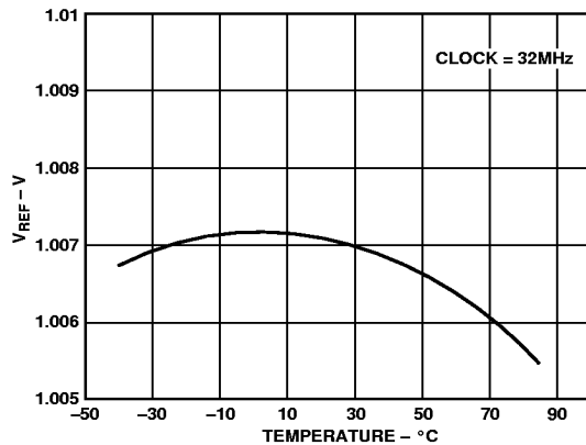
Figure 9. Voltage Reference Error vs. Temperature
