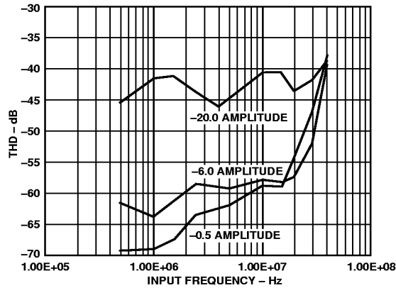
Figure 7. THD vs. Input Frequency
