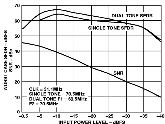
Figure 36. SNR/SFDR for IF @ 70 MHz
