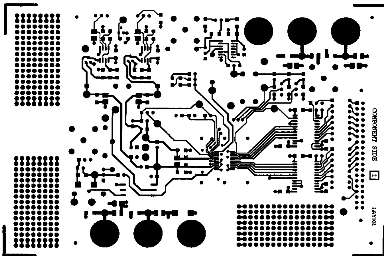
Figure 40a. Evaluation Board, Component Signal (Not to Scale)
