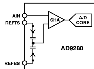
Figure 15. AD9280 Equivalent Functional Input Circuit
