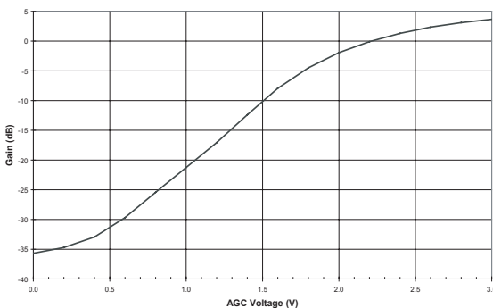
Figure 8: Gain vs. AGC Voltage (T C = +25 °C, V DD = +5 V, at 495 MHz)
