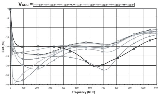
Figure 6: Output Return Loss (S22) vs. Frequency (T C = +25 °C, V DD = +5 V)
