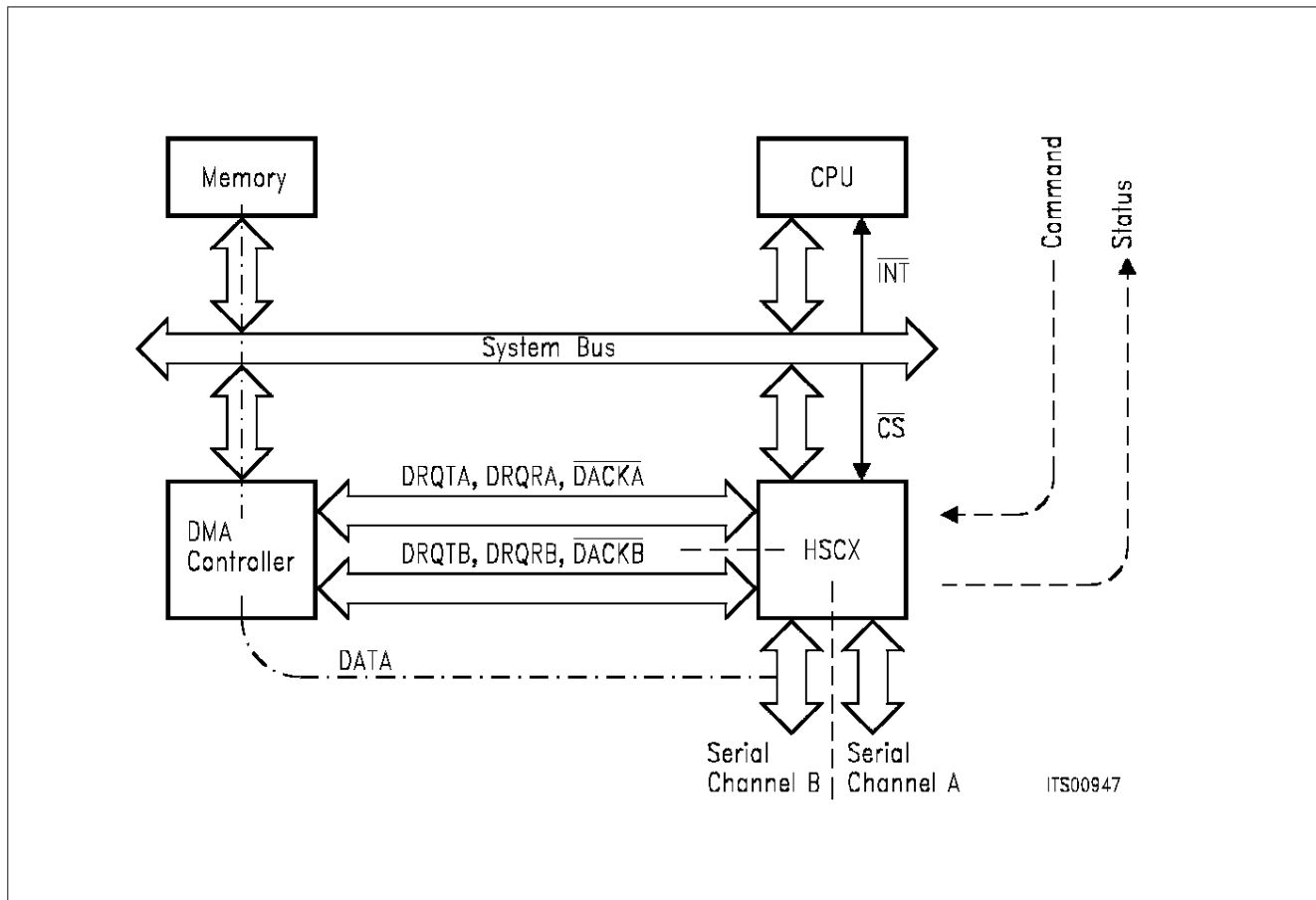
Figure 2 General System Integration of HSCX
