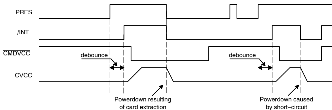
Figure 7. Fault Detection and Interrupt Management
