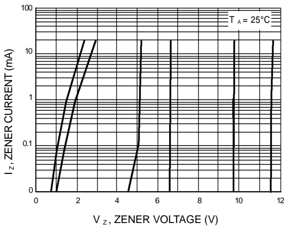
V_Z , ZENER VOLTAGE (V) Figure 7. Zener Voltage versus Zener Current ( V_Z Up to 12 V)
