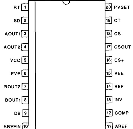
SOIC-20 (Top View) DW Package
