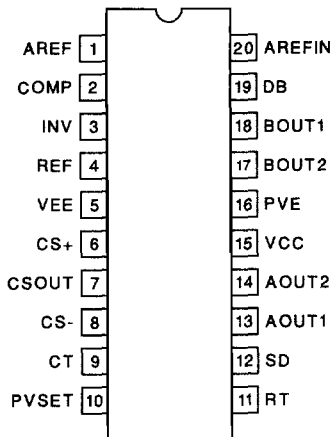
DIL-20 (Top View) N or J Package
