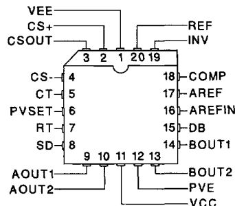
PLCC-20 (Top View) Q Package
