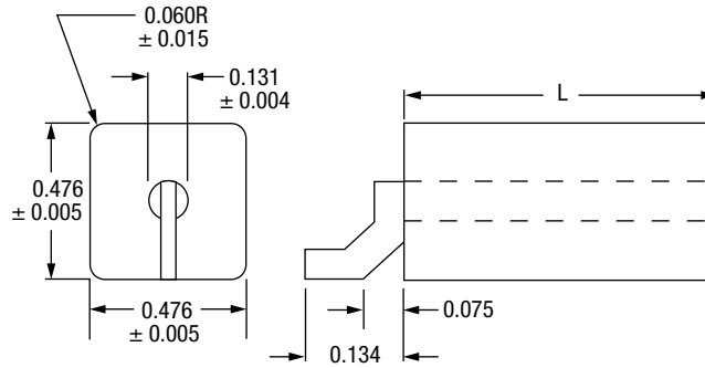
Figure 1.3g. HP – High Profile (12 mm)
