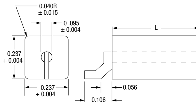
Figure 1.3e. SP – Standard Profile (6 mm)
