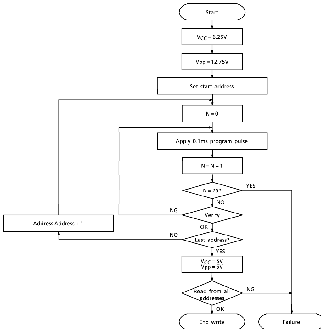
Figure Write Flow Chart in High-Speed Program Mode II
