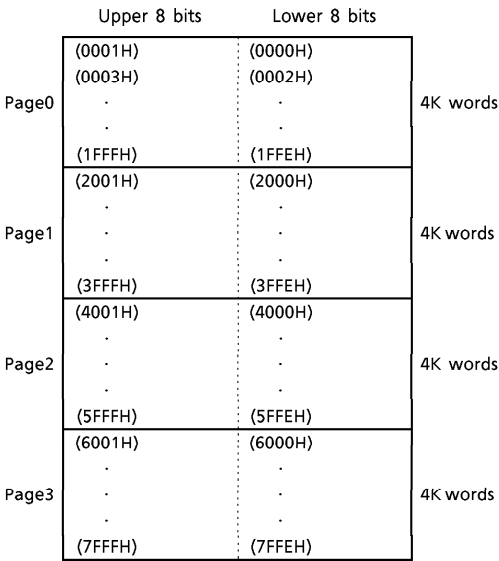
Figure 2 Addresses in PROM Mode
