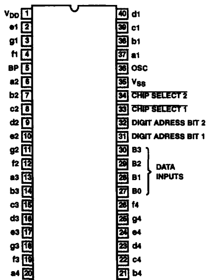
ICM7211M, ICM7211AM (PDIP) TOP VIEW
