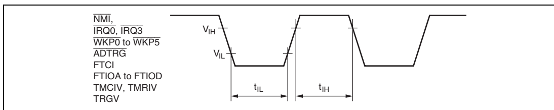
Figure 17.3 Input Timing
