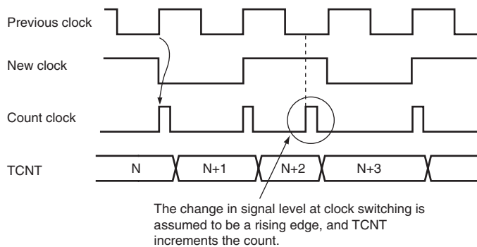
Figure 11.25 Internal Clock Switching and TCNT Operation
