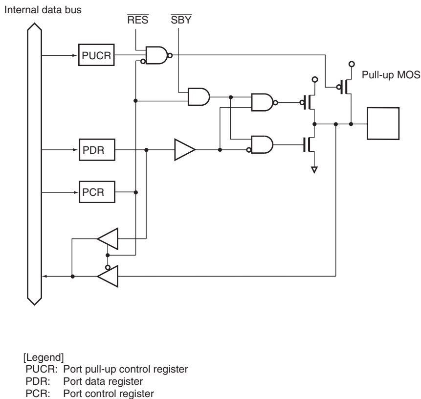
Figure B.4 Port 1 Block Diagram (P11)
