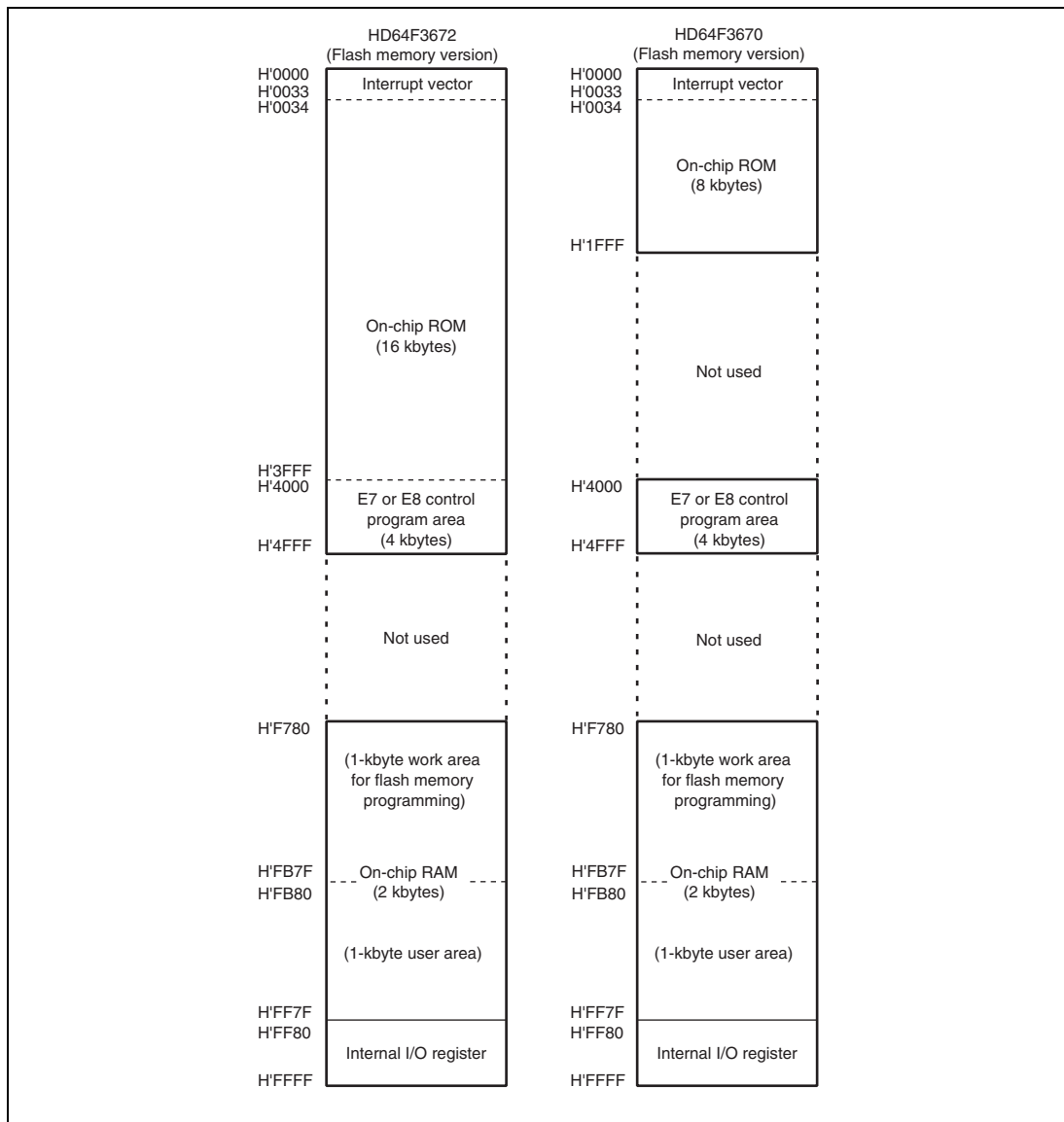
Figure 2.1 Memory Map
