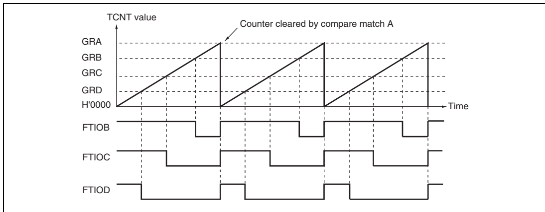
Figure 11.9 PWM Mode Example (1)
