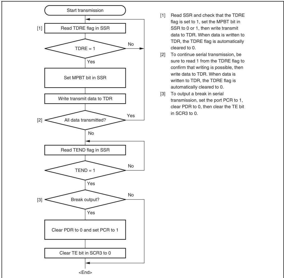
Figure 13.16 Sample Multiprocessor Serial Transmission Flowchart
