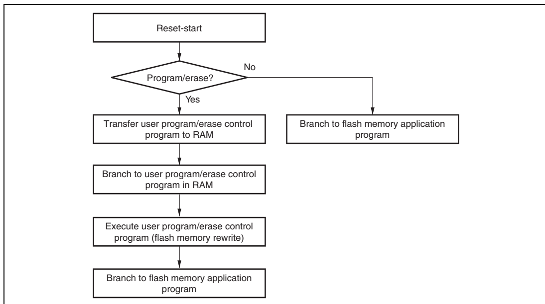
Figure 7.2 Programming/Erasing Flowchart Example in User Program Mode
