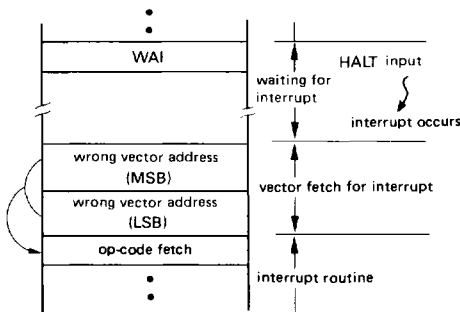
Figure 39 MAC function during WAI
