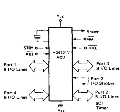
Figure 15 HD6301V1 MCU Single-Chip Mode
