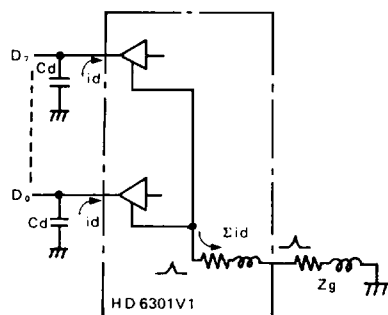
Fig. 34 Noise Source
