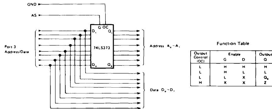
Figure 18 Latch Connection
