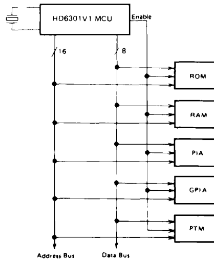
Figure 30 HD6301V1 MCU Expanded Non-Multiplexed Mode (Mode 1)
