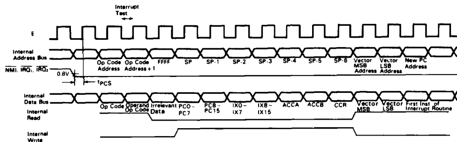
Figure 10 Interrupt Sequence
