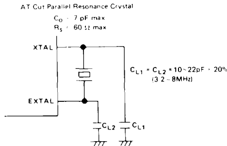
Figure 12 Crystal Interface
