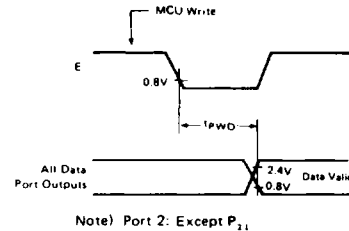
Note) Port 2: Except P 21 Figure 4 Port Data Delay Times (MCU Write)
