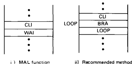
Figure 40 Program to wait for interrupt
