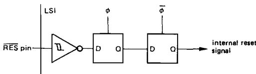
Figure 41 RES circuit
