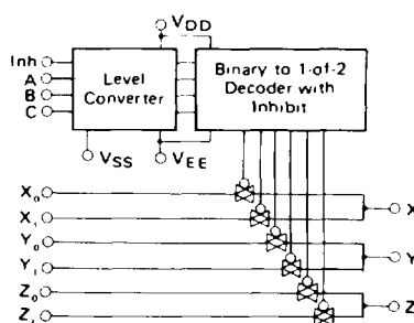
Figure 14 HD14053B Multiplexers/De-Multiplexers
