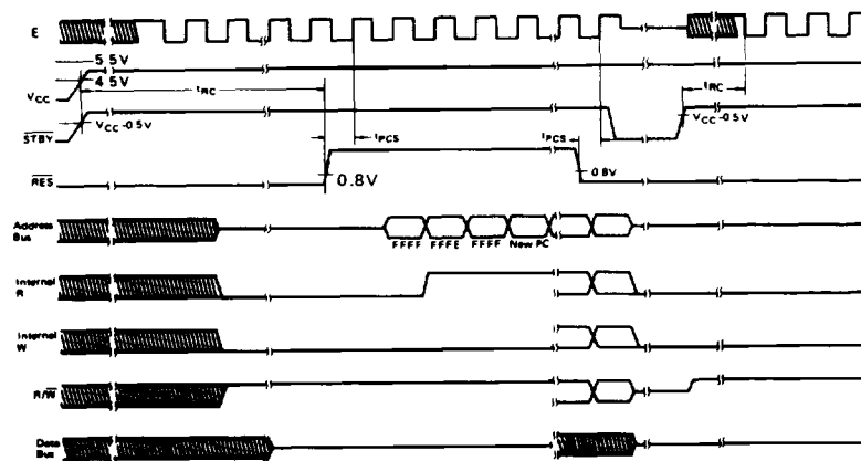
Figure 11 Reset Timing
