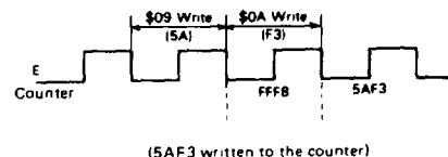
Figure 21 Counter Write Timing
