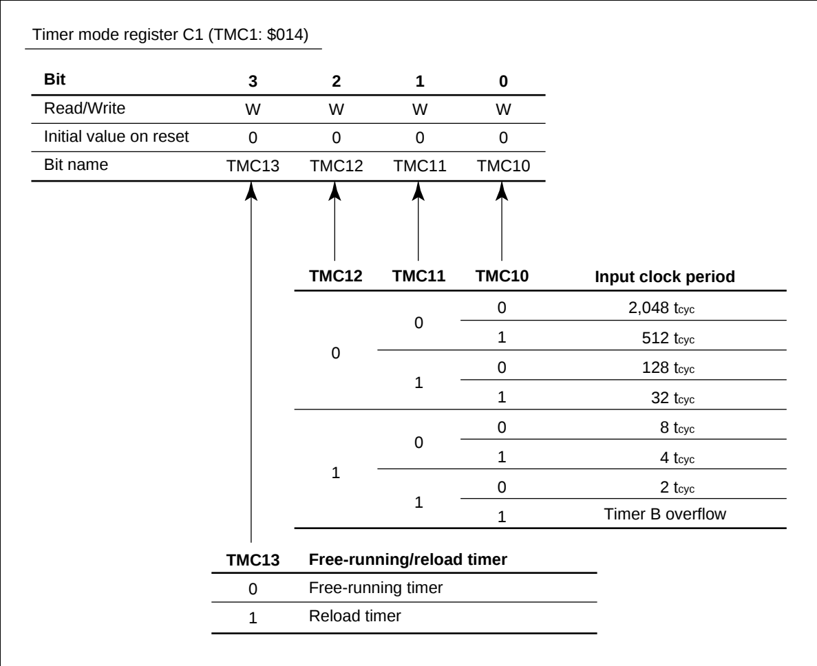
Figure 48 Timer Mode Register C1 (TMC1)
