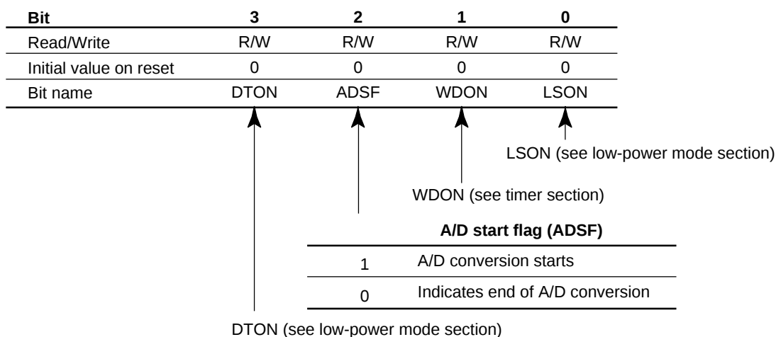
Figure 81 A/D Start Flag (ADSF)
