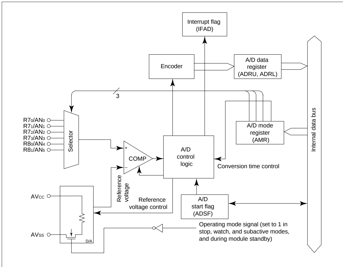
Figure 73 A/D Converter Block Diagram
