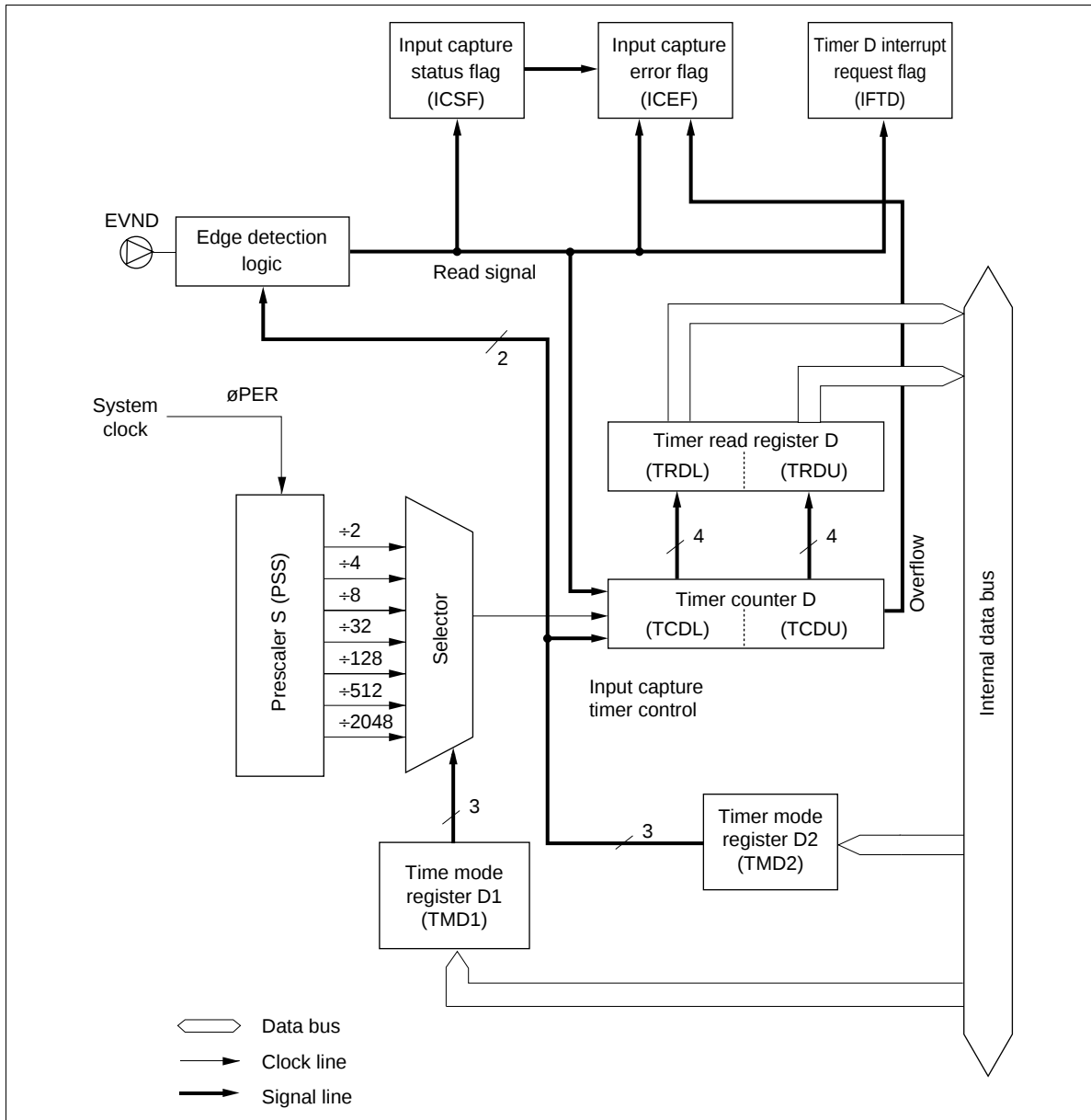
Figure 55-2 Timer D Block Diagram (Input Capture Timer Mode)
