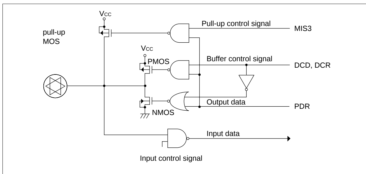
Figure 26 I/O Pin Circuit Configuration
