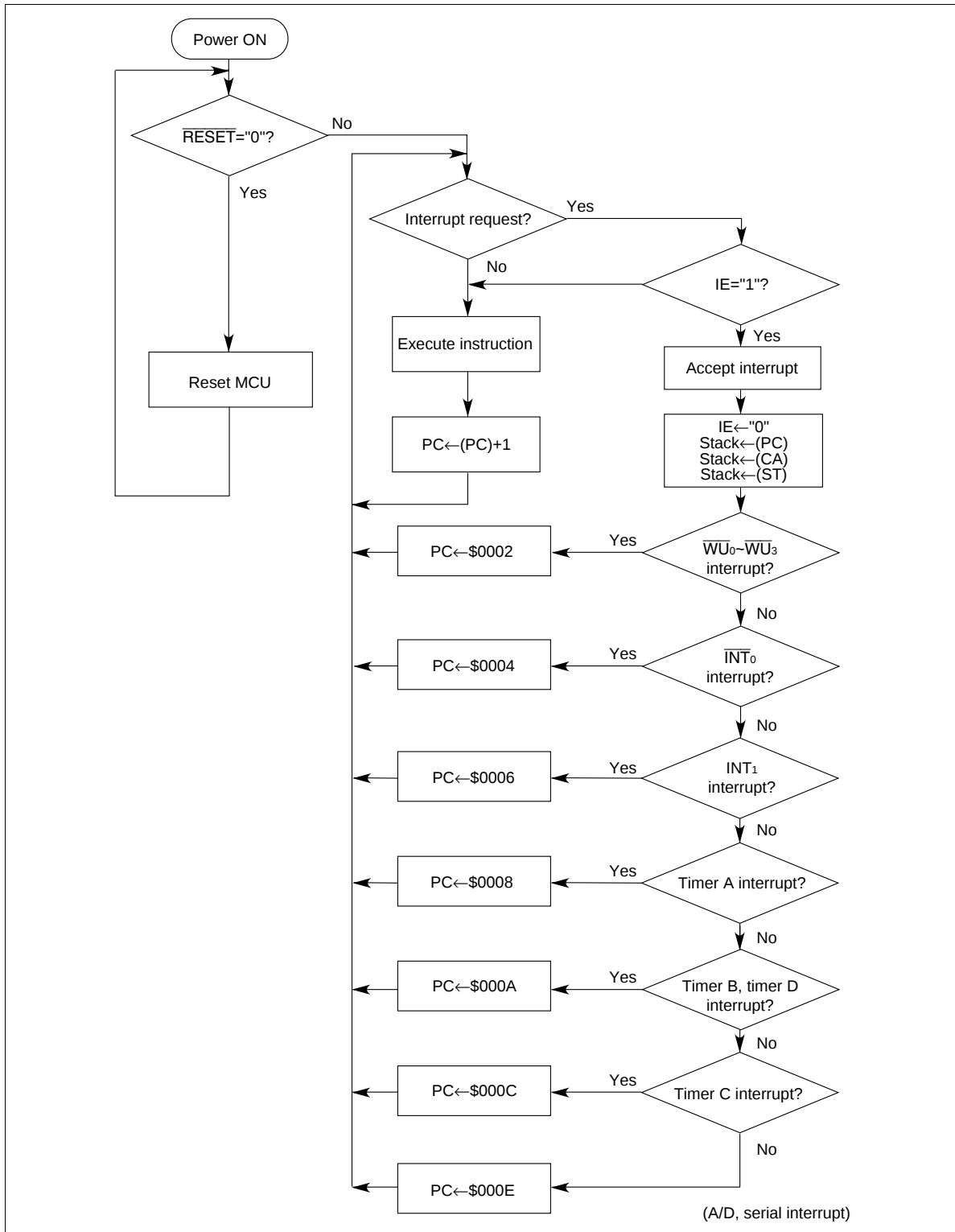
Figure 11 Interrupt Handling Flowchart
