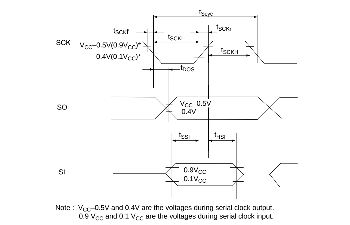
Figure 107 Serial Interface Timing
