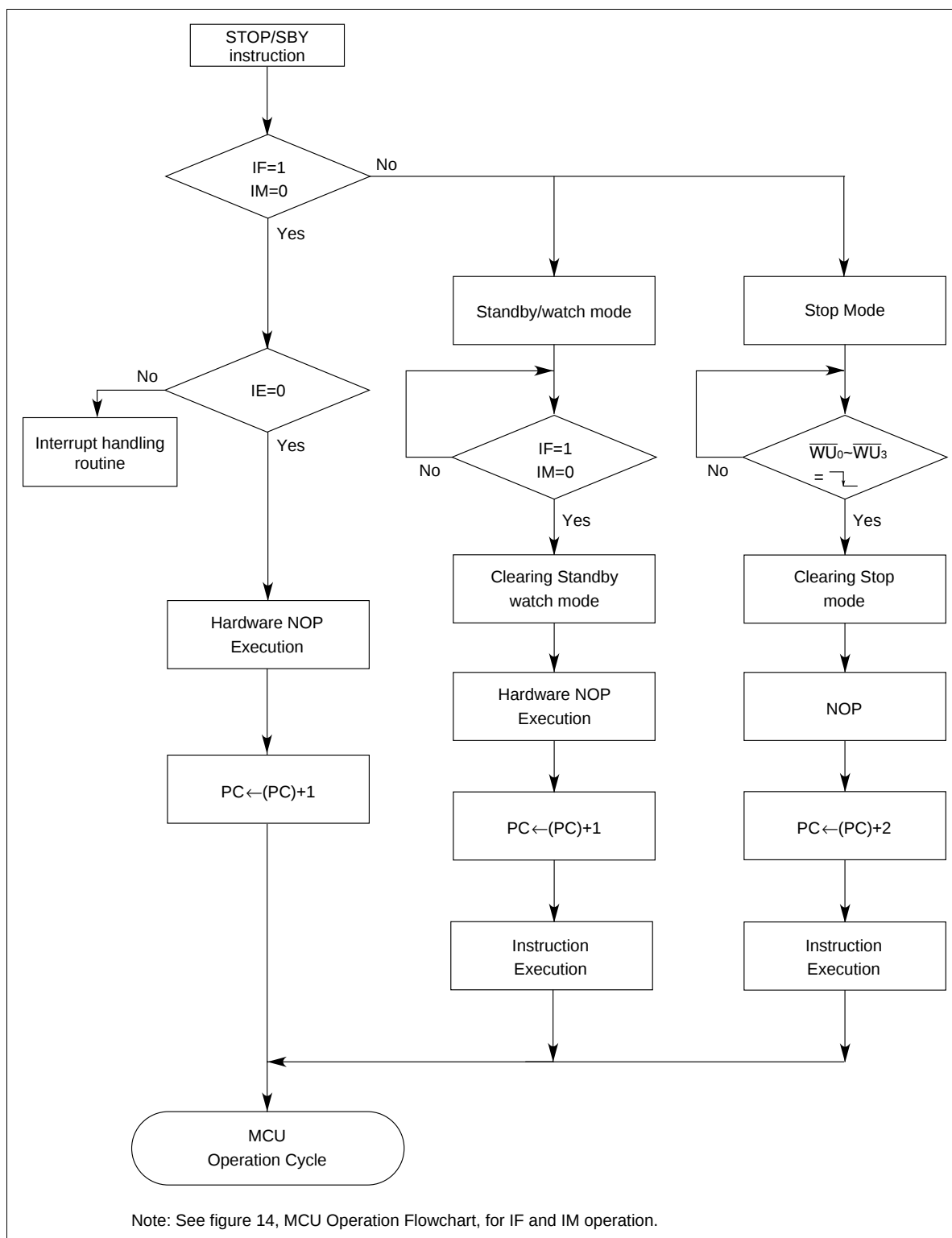
Figure 19 MCU Operating Sequence (Low-Power Mode Operation)
