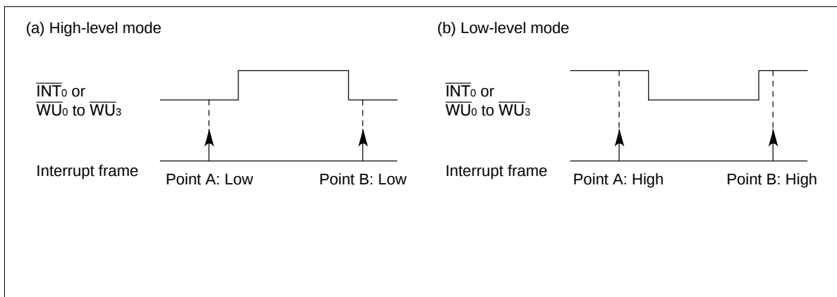
Figure 21 Sampling Examples
