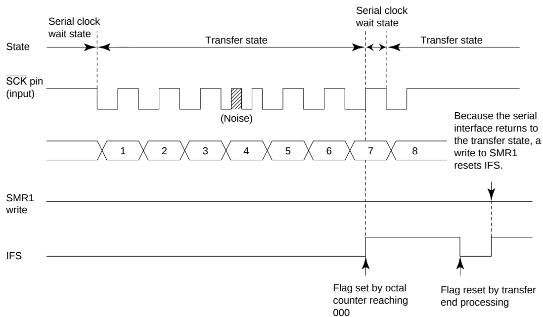
(2) Serial clock error detection sequence
