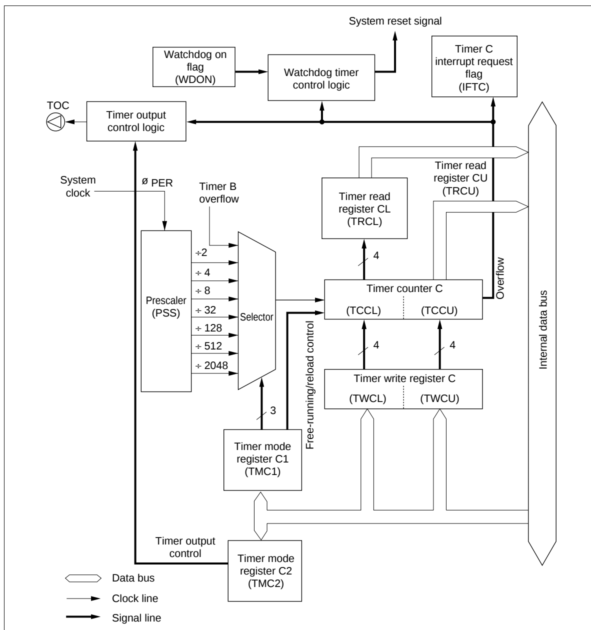
Figure 47 Timer C Block Diagram
