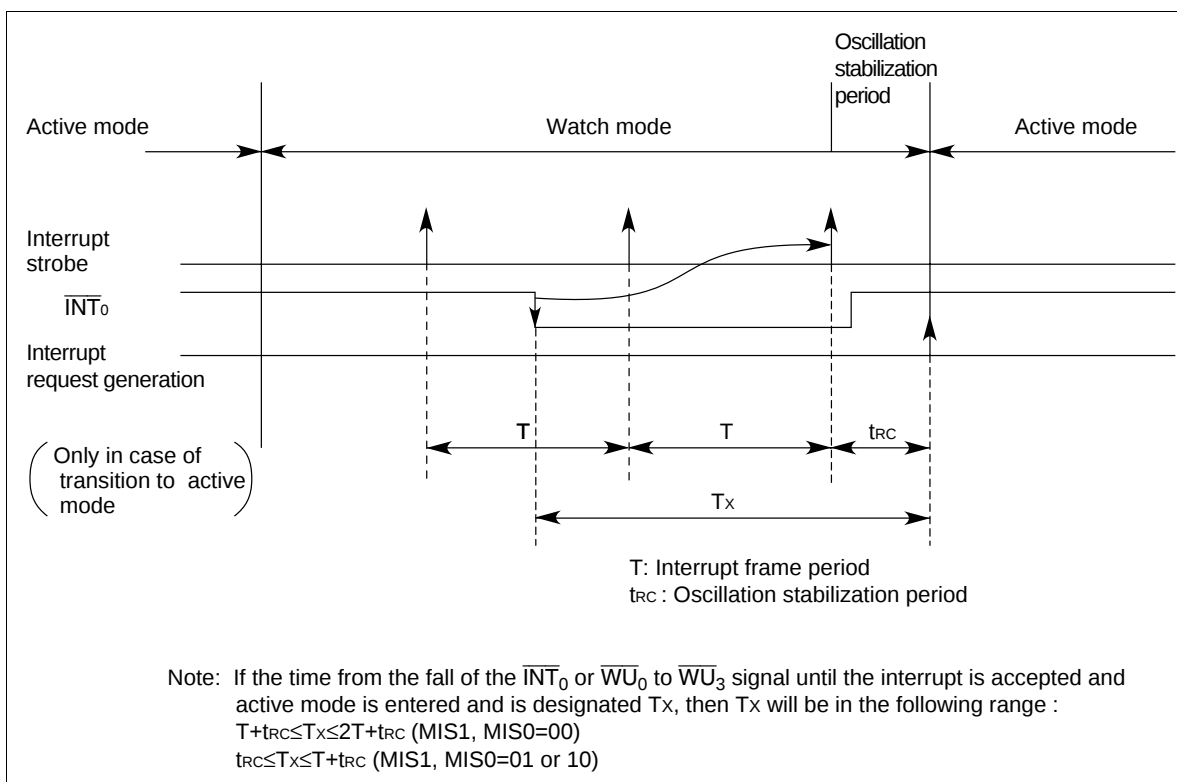
Figure 16 Interrupt Frame
