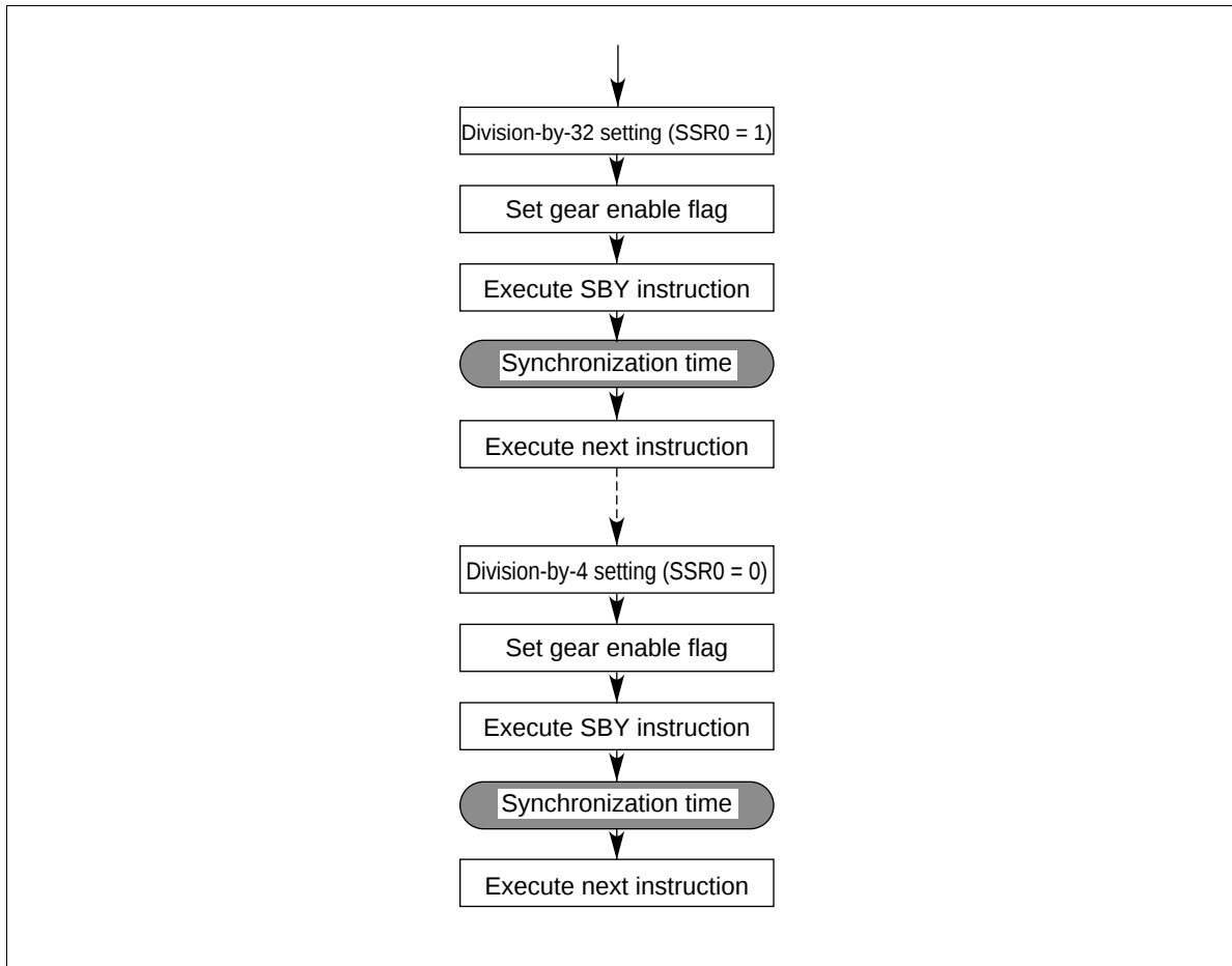
Figure 23 System Clock Division Ratio Conversion Flowchart
