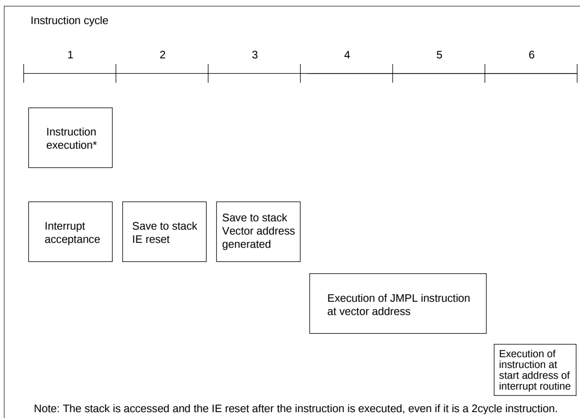
Figure 10 Interrupt Sequence
