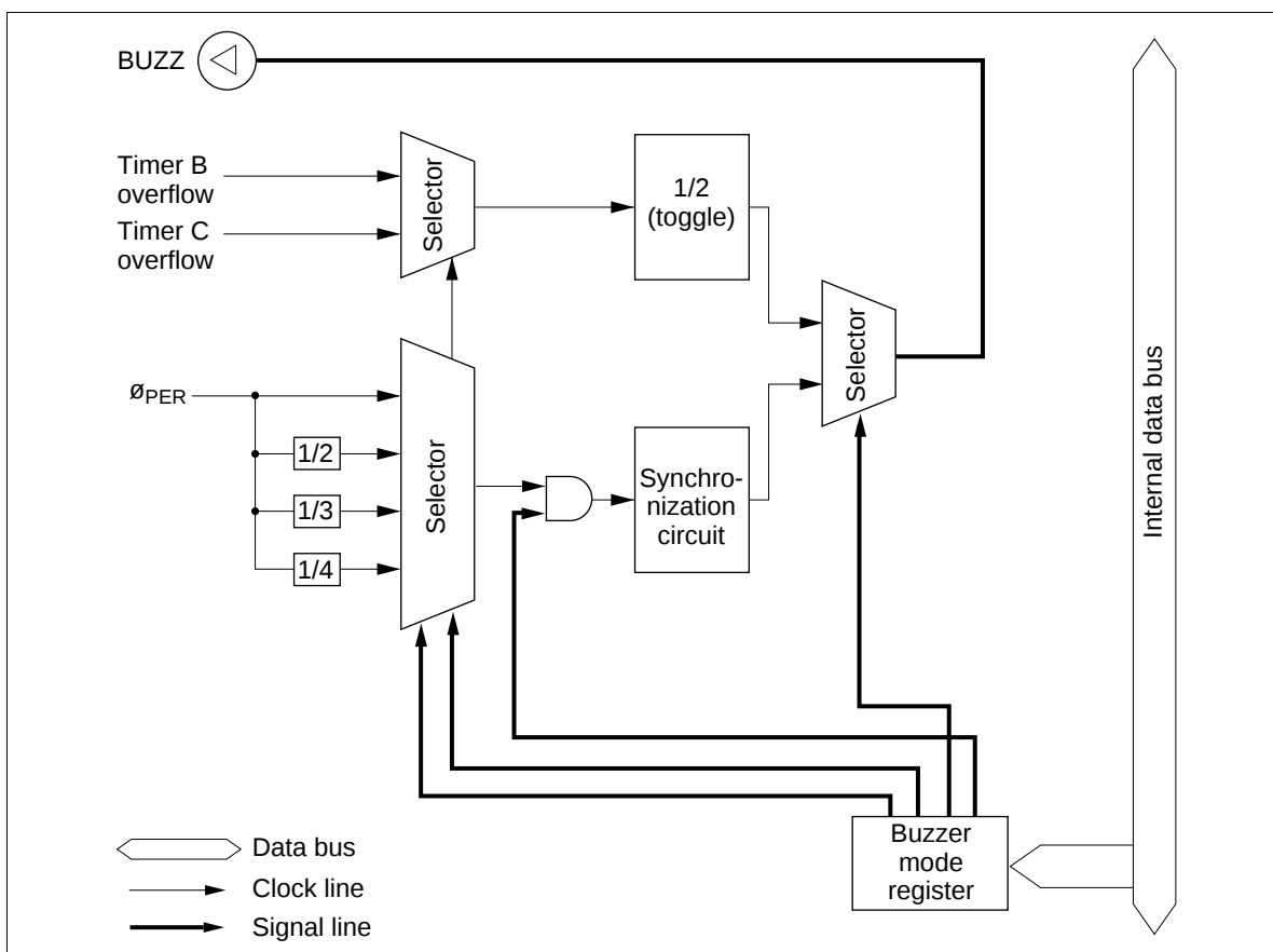
Figure 93 Buzzer Output Circuit
