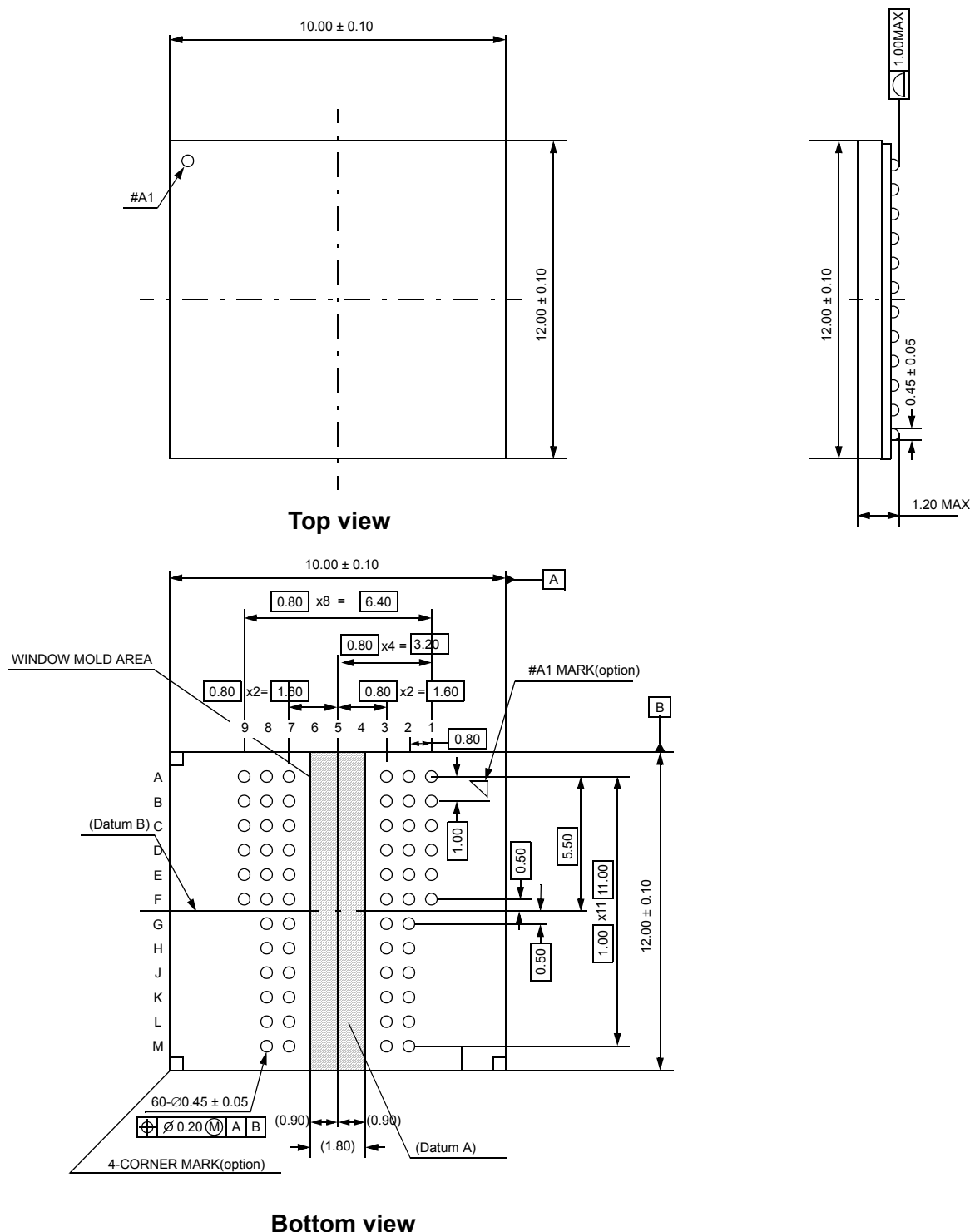
60Ball FBGA 512Mb Package Dimension
