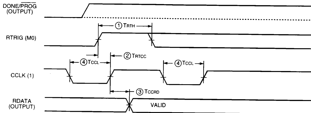
Figure 40. Program Readback Switching Characteristics
