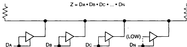
Figure 15A. 3-State Buffers Implement a Wired-AND Function
