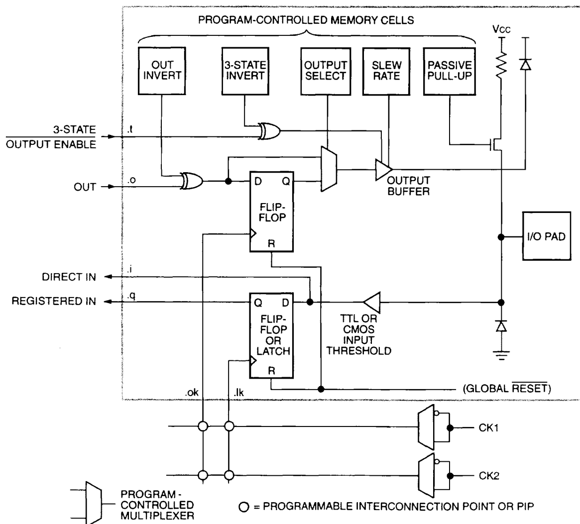
Figure 3. Input/Output Block
