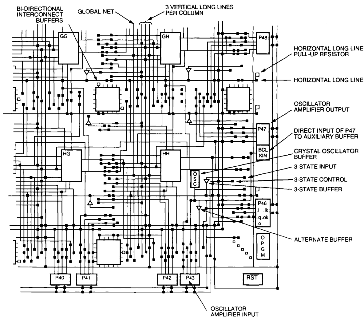
Figure 15B. 3-State Buffers Implement a Multiplexer
