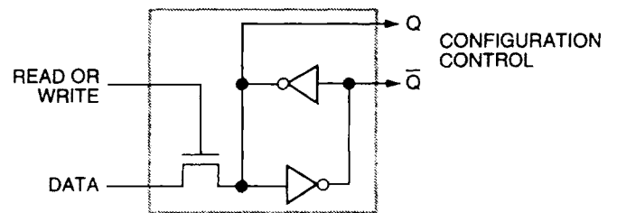
Figure 1. Static Configuration Memory Cell
