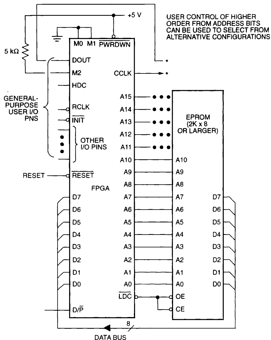
Figure 22. Master Parallel Mode
