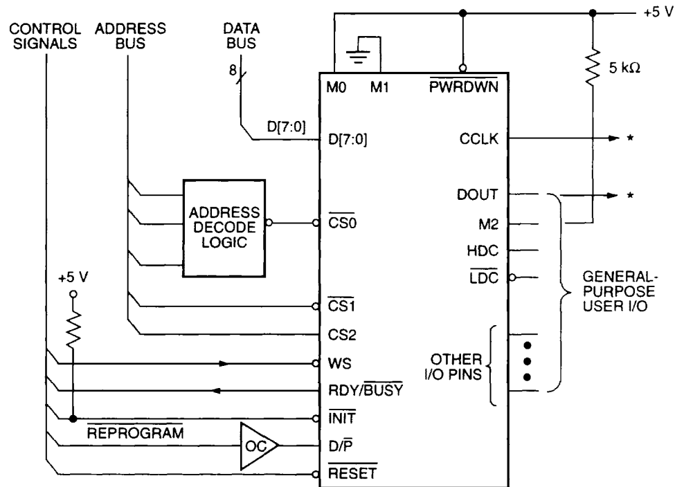
Figure 23. Peripheral Mode
