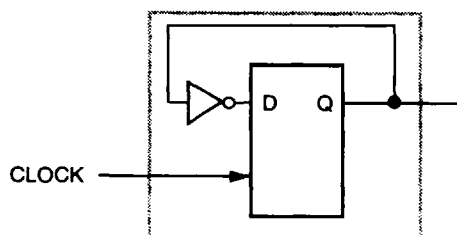
Figure 26. Toggle Flip-Flop
