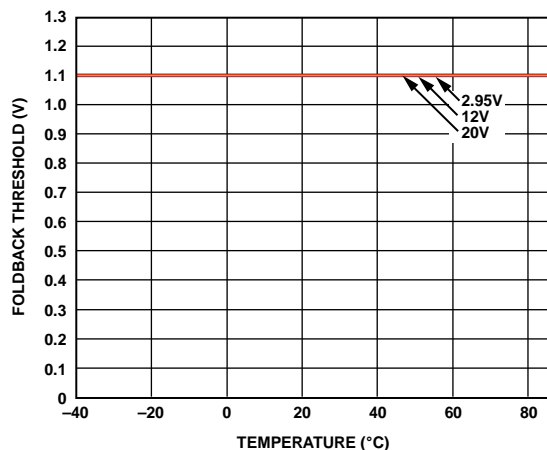
Figure 20. Foldback Threshold vs. Temperature
