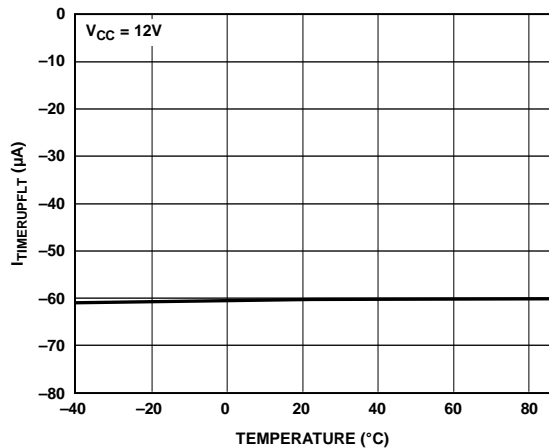
Figure 16. Timer Pull-Up Current, Overcurrent Fault ( I_{TIMERUPFLT} ) vs. Temperature
