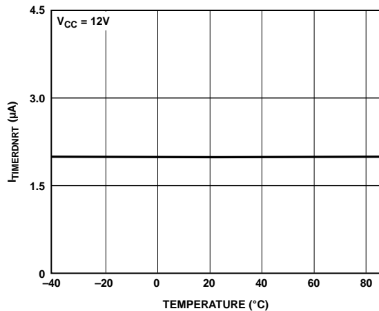
Figure 18. Timer Pull-Down Current, Retry ( I_{TIMERDNRT} ) vs. Temperature
