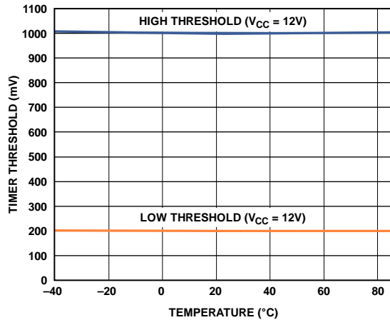
Figure 19. Timer Thresholds vs. Temperature
