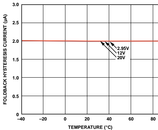
Figure 21. Foldback Hysteresis Current vs. Temperature
