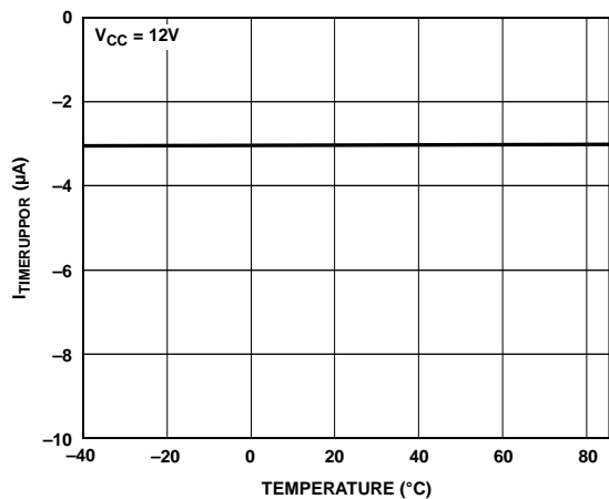
Figure 17. Timer Pull-Up Current, Power-On Reset ( I_{TIMERUPPOR} ) vs. Temperature
